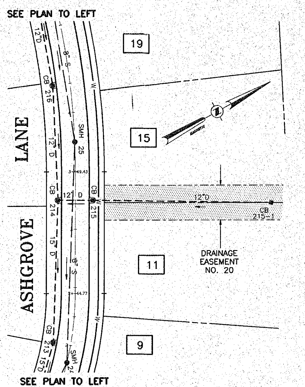
2 PLAN - CB215-1 TO CB215 STA 0+00 TO STA 1+54 SCALE: 1" = 50' CROSS REFERENCE: NONE
