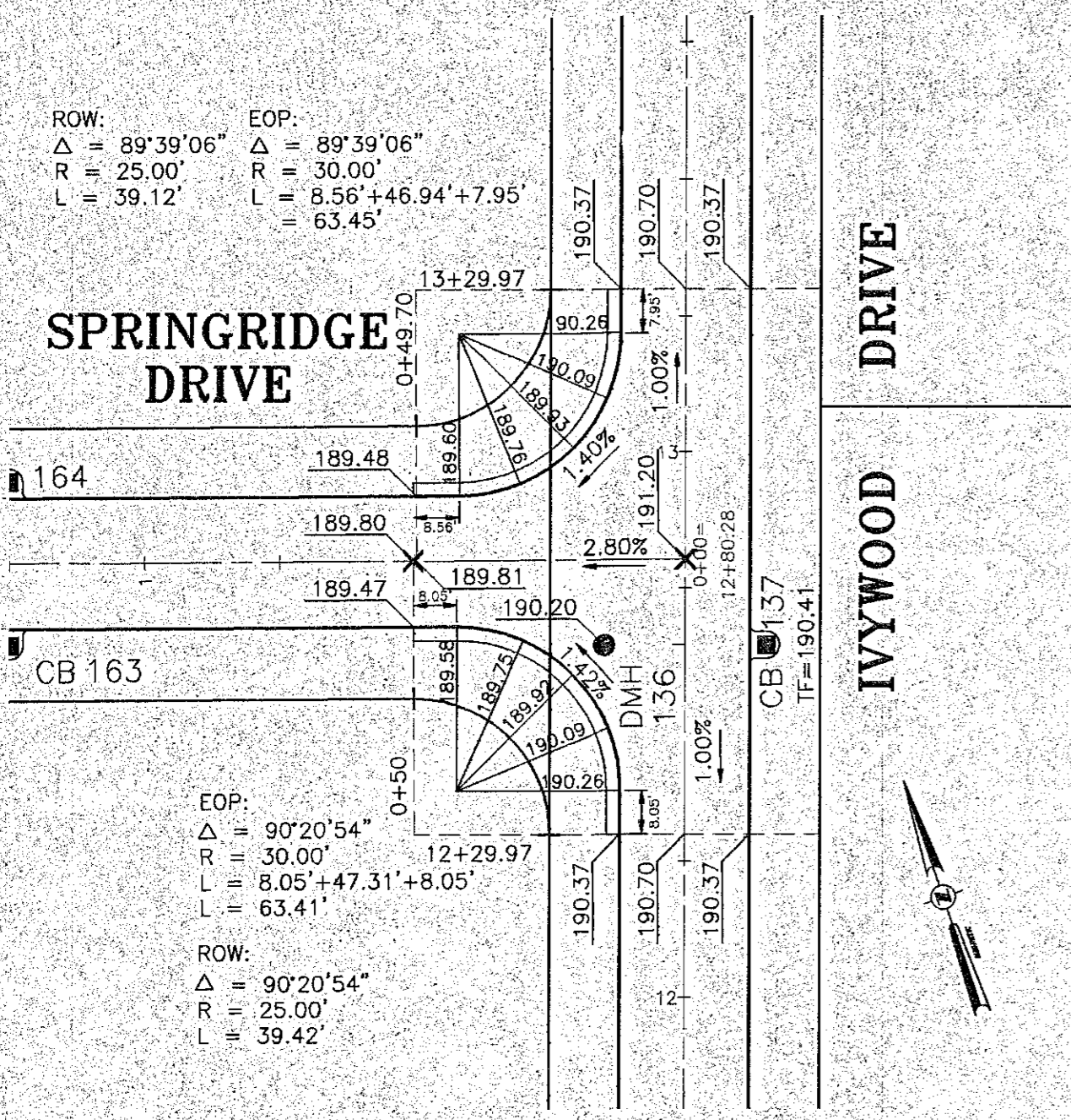
INTERSECTION DETAIL SPRINGRIDGE DR & IVYWOOD DR
