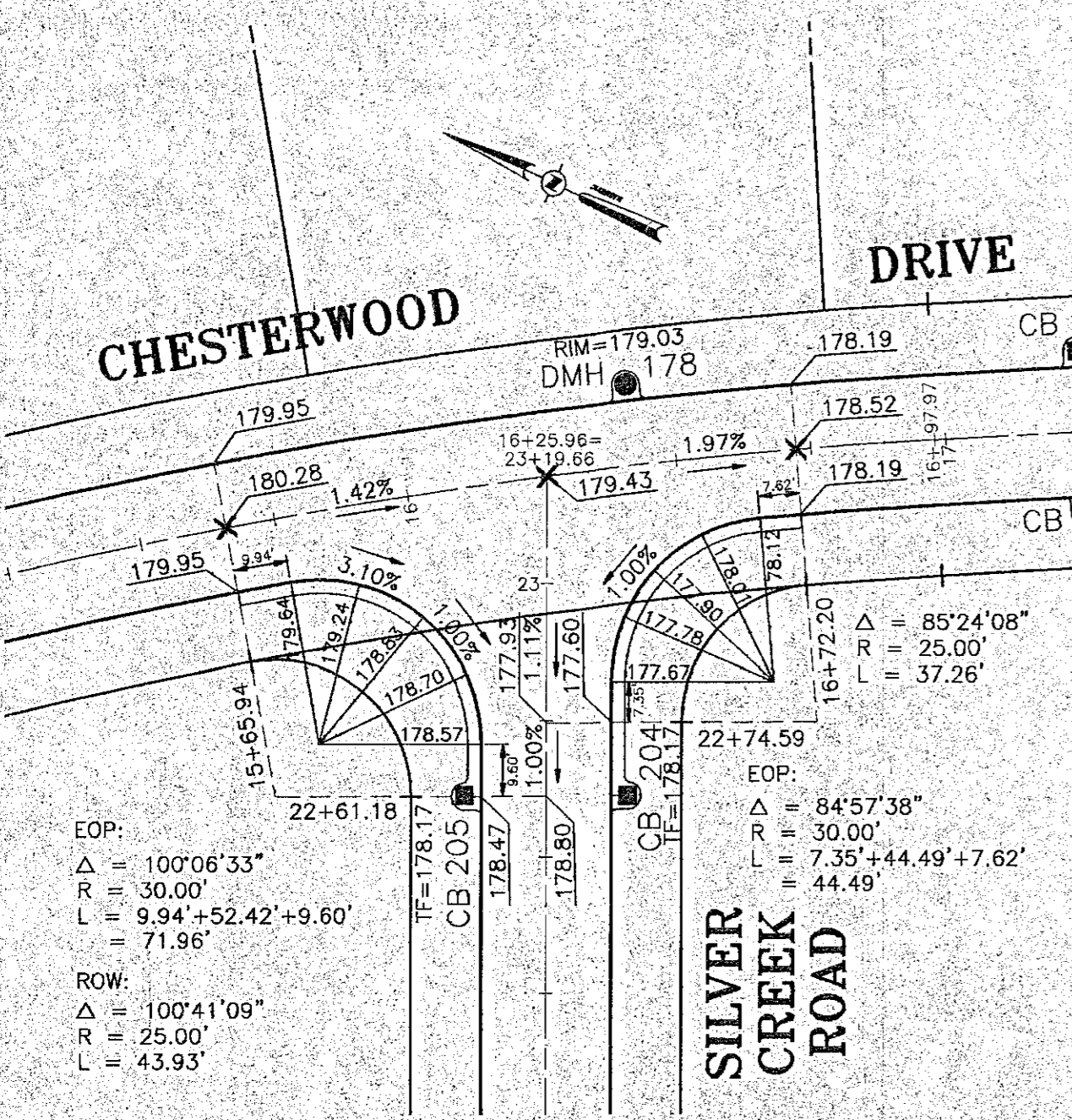
INTERSECTION DETAIL CHESTERWOOD DR & SILVER CREEK DR
