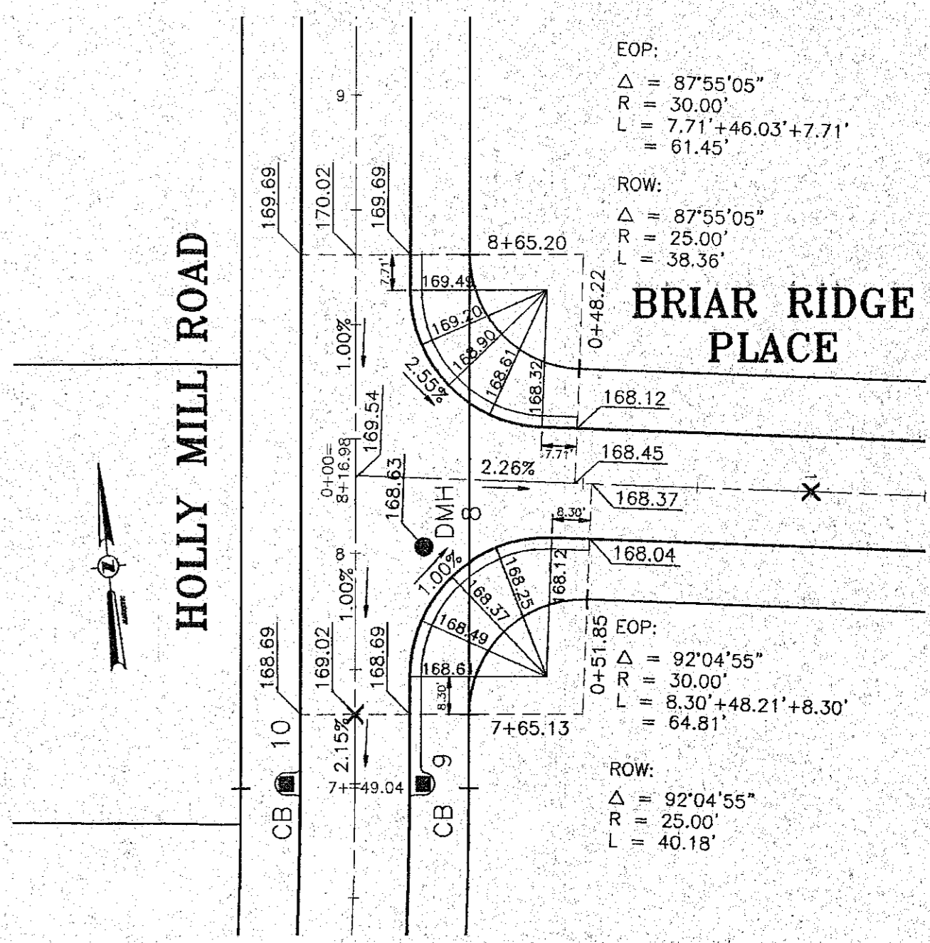
INTERSECTION DETAIL HOLLY MILL RD & BRIAR RIDGE PLACE
