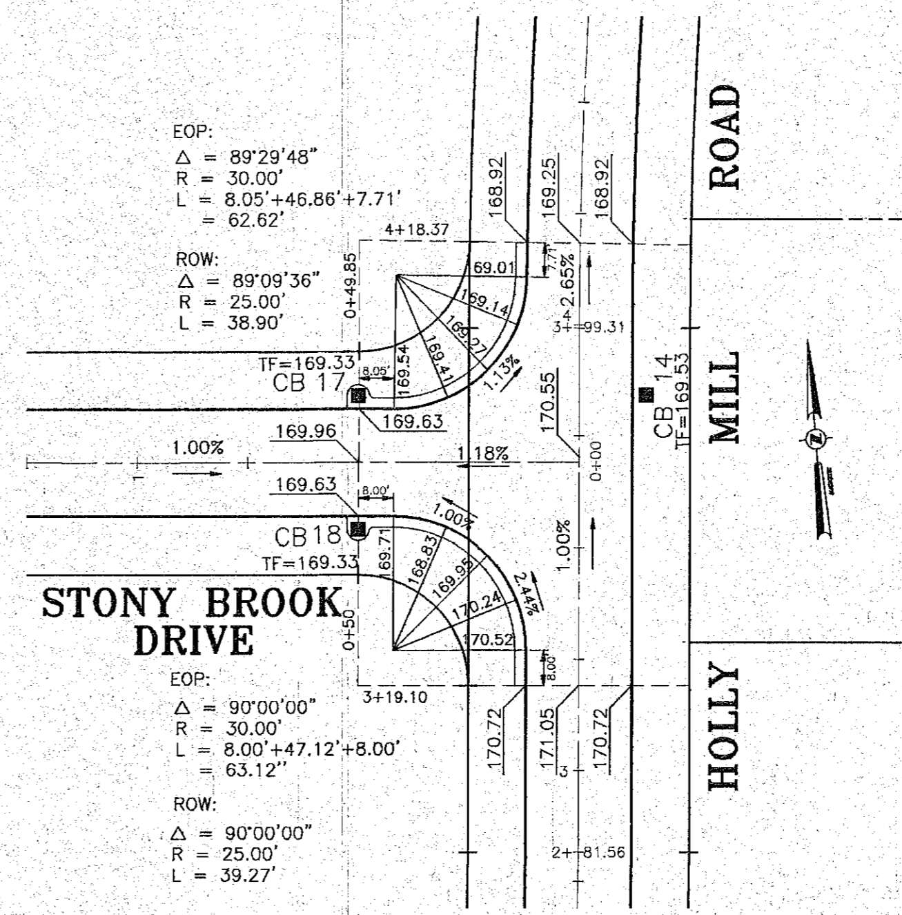
INTERSECTION DETAIL STONY BROOK DR & HOLLY MILL RD
