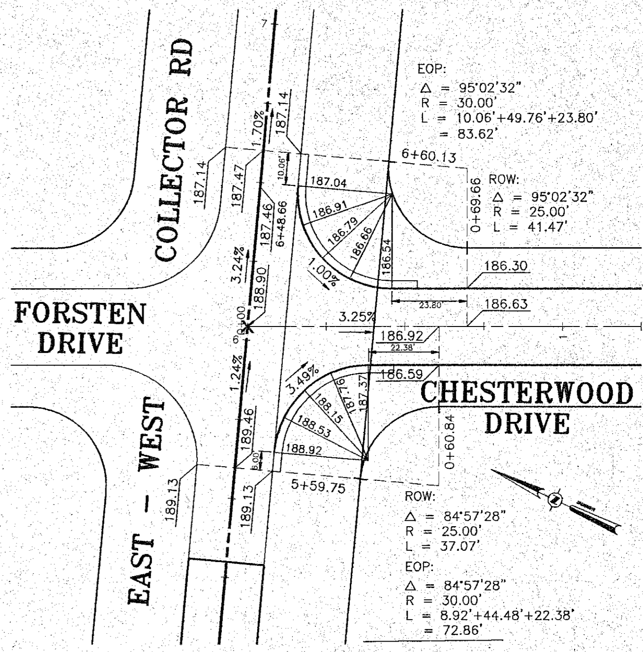
INTERSECTION DETAIL CHESTERWOOD DR & EAST-WEST COLLECTOR
