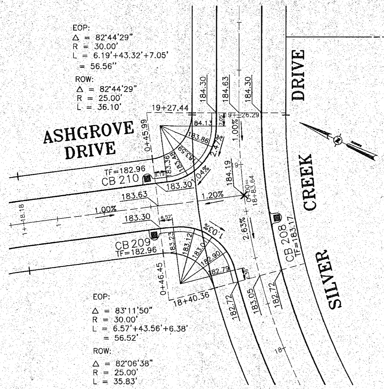
INTERSECTION DETAIL ASHGROVE DR & SILVER CREEK DR
