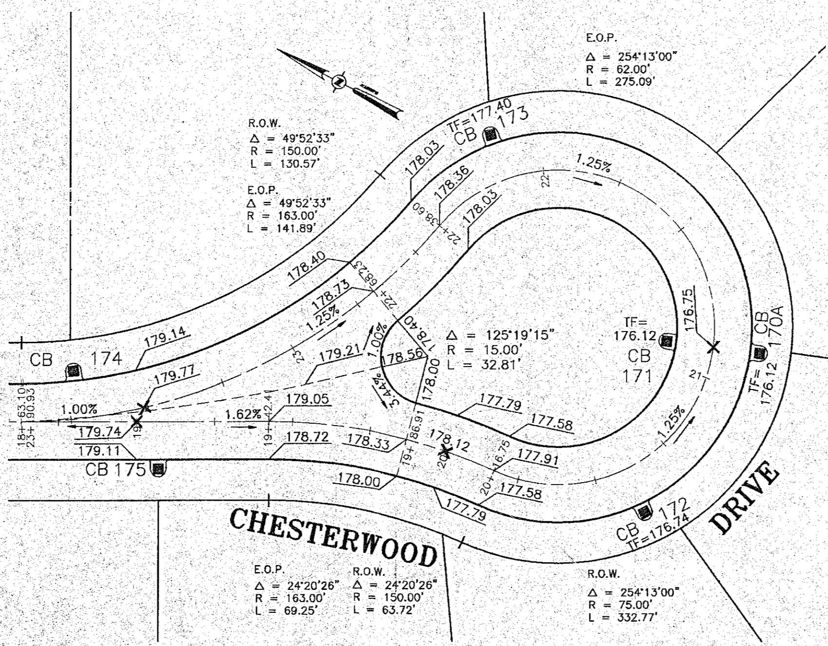
CUL-DE-SAC DETAIL CHESTERWOOD DR
