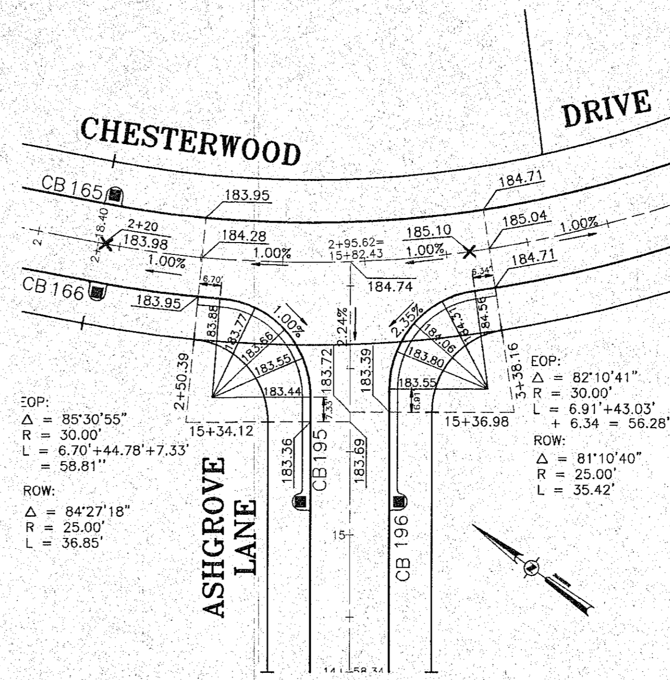
INTERSECTION DETAIL CHESTERWOOD DR & ASHGROVE LN
