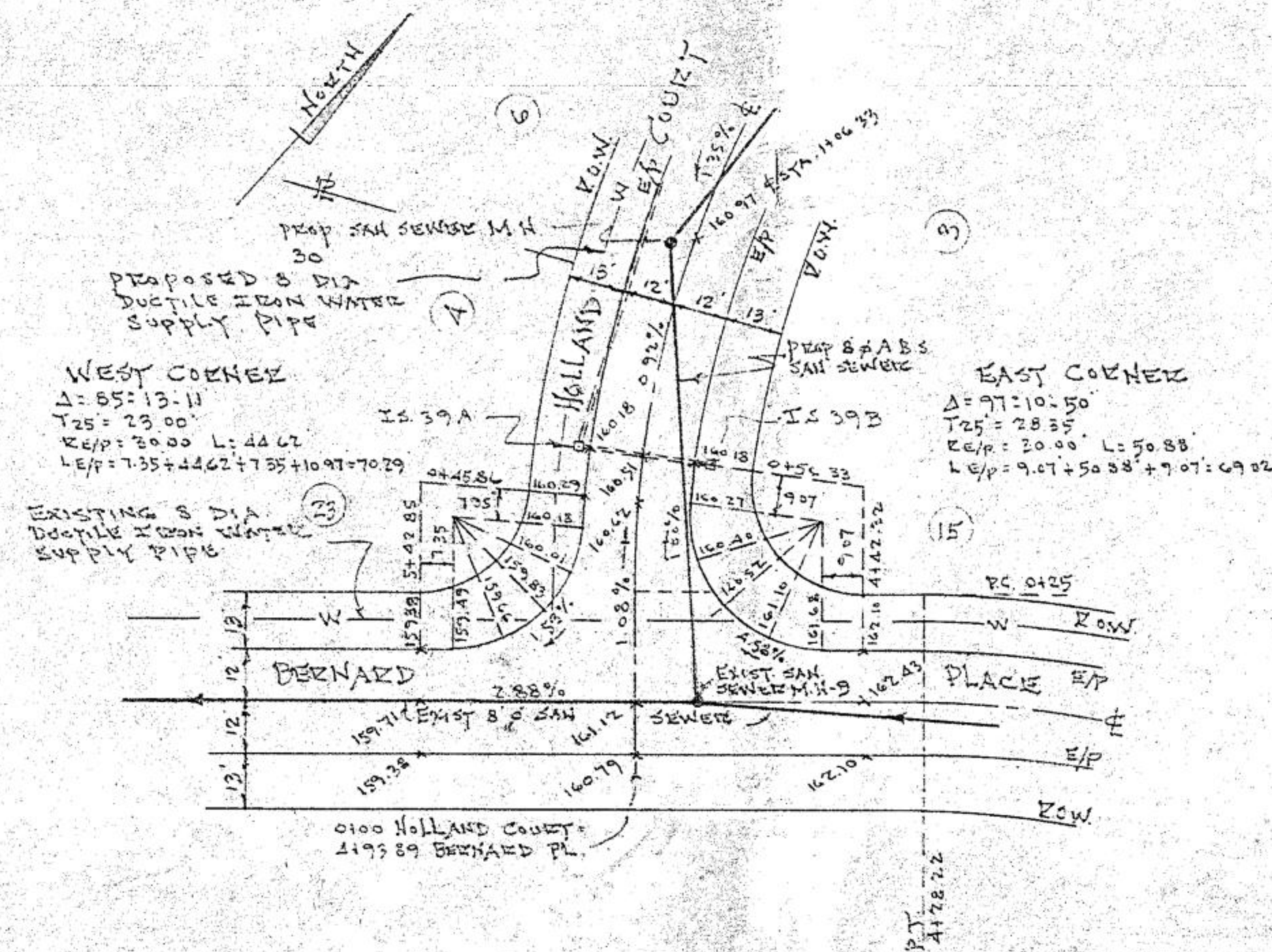
BERNARD PLACE & HOLLAND COURT INTERSECTION SCALE: 1" = 30'
