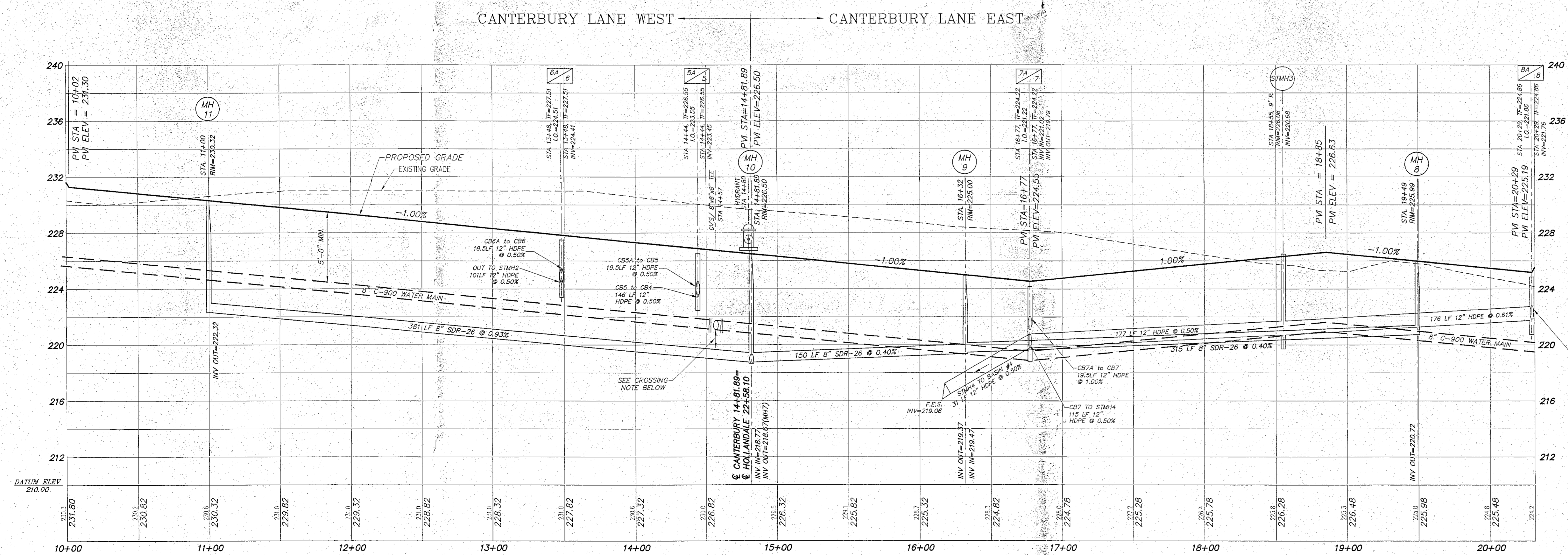
PROFILE HOR: 1" = 40' VER: 1" = 4'
