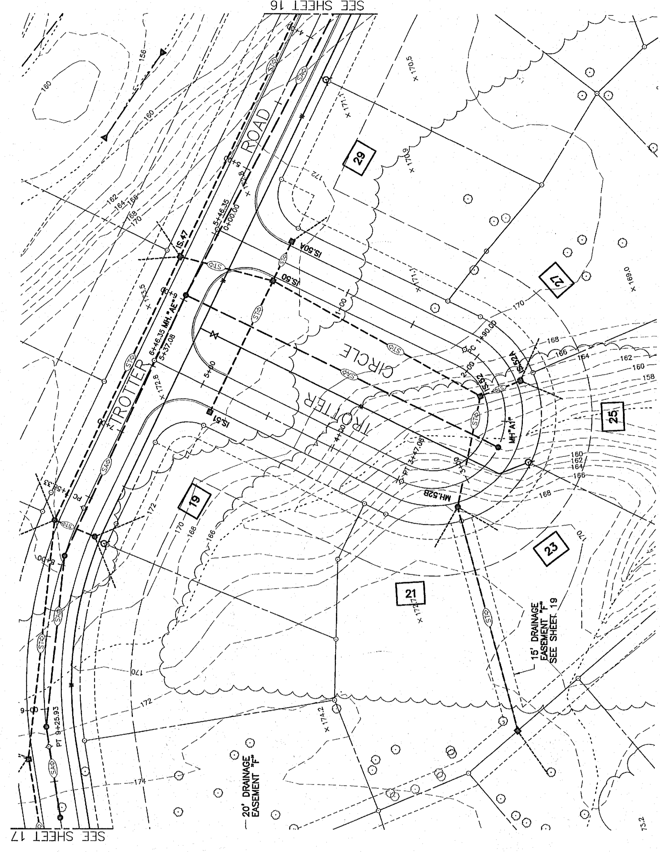
GENERAL PLAN - TROTTER CIRCLE SCALE: 1" = 40'
