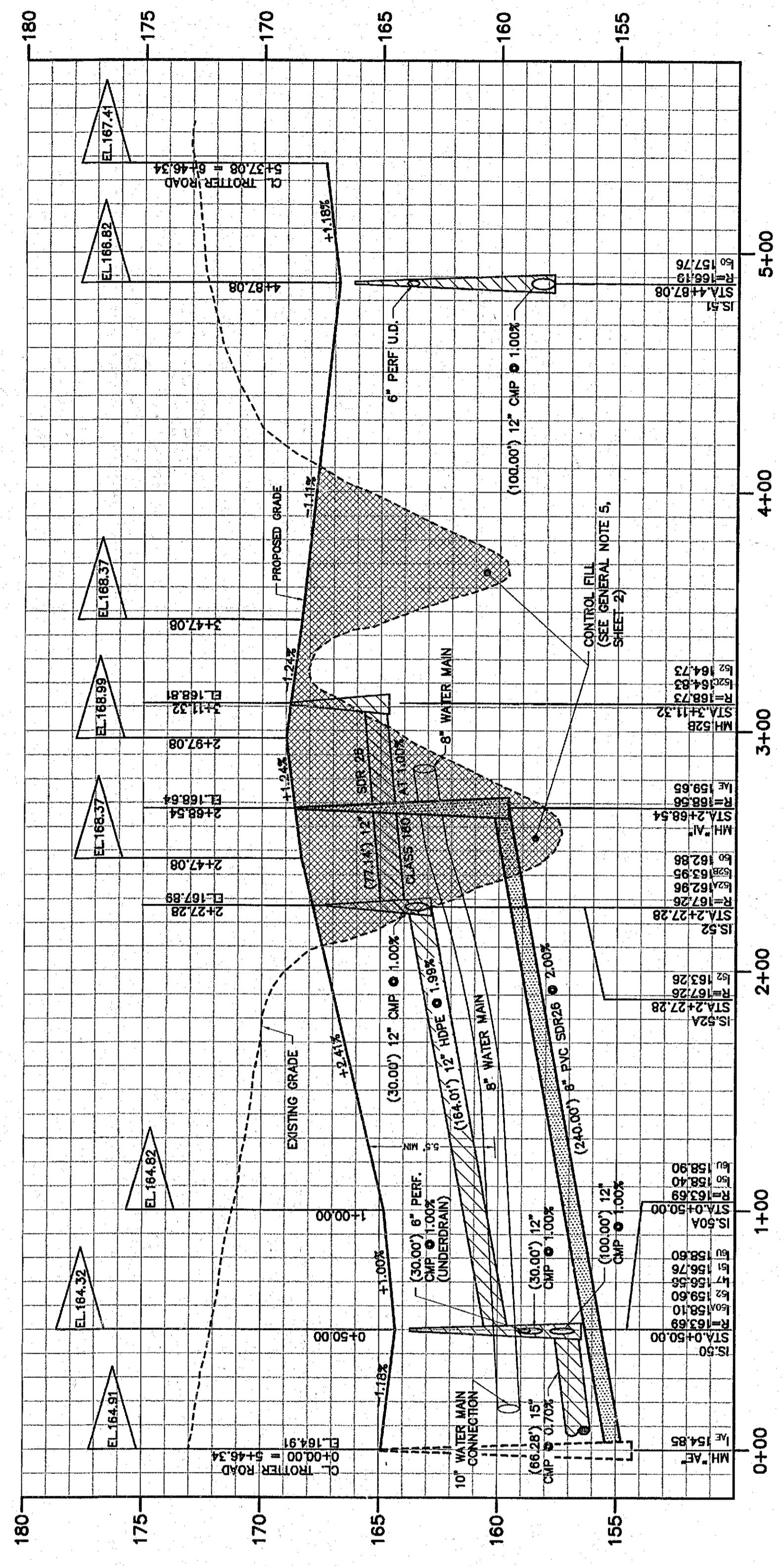
PROFILE - TROTTER CIRCLE SCALE: 1" = 4' VERT. / 1" = 40' HORIZ.
