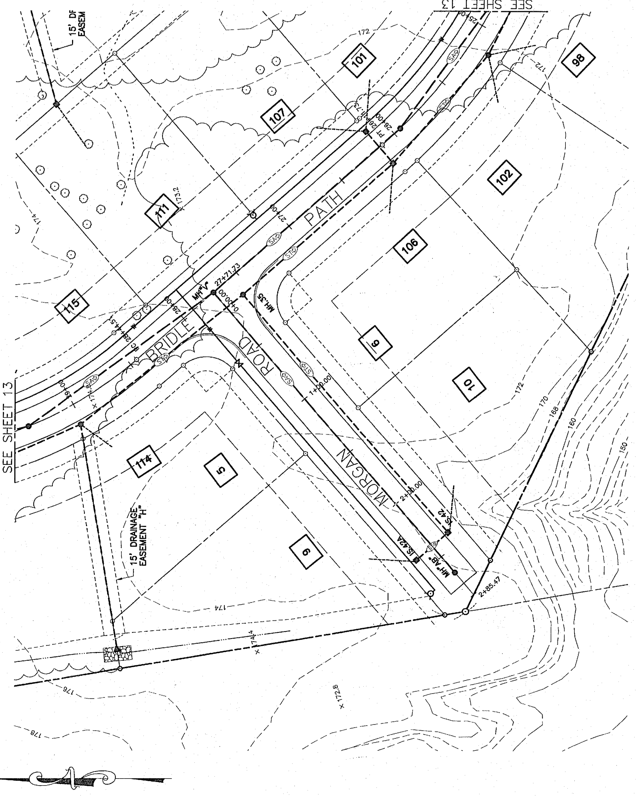
GENERAL PLAN - MORGAN ROAD SCALE: 1" = 40'
