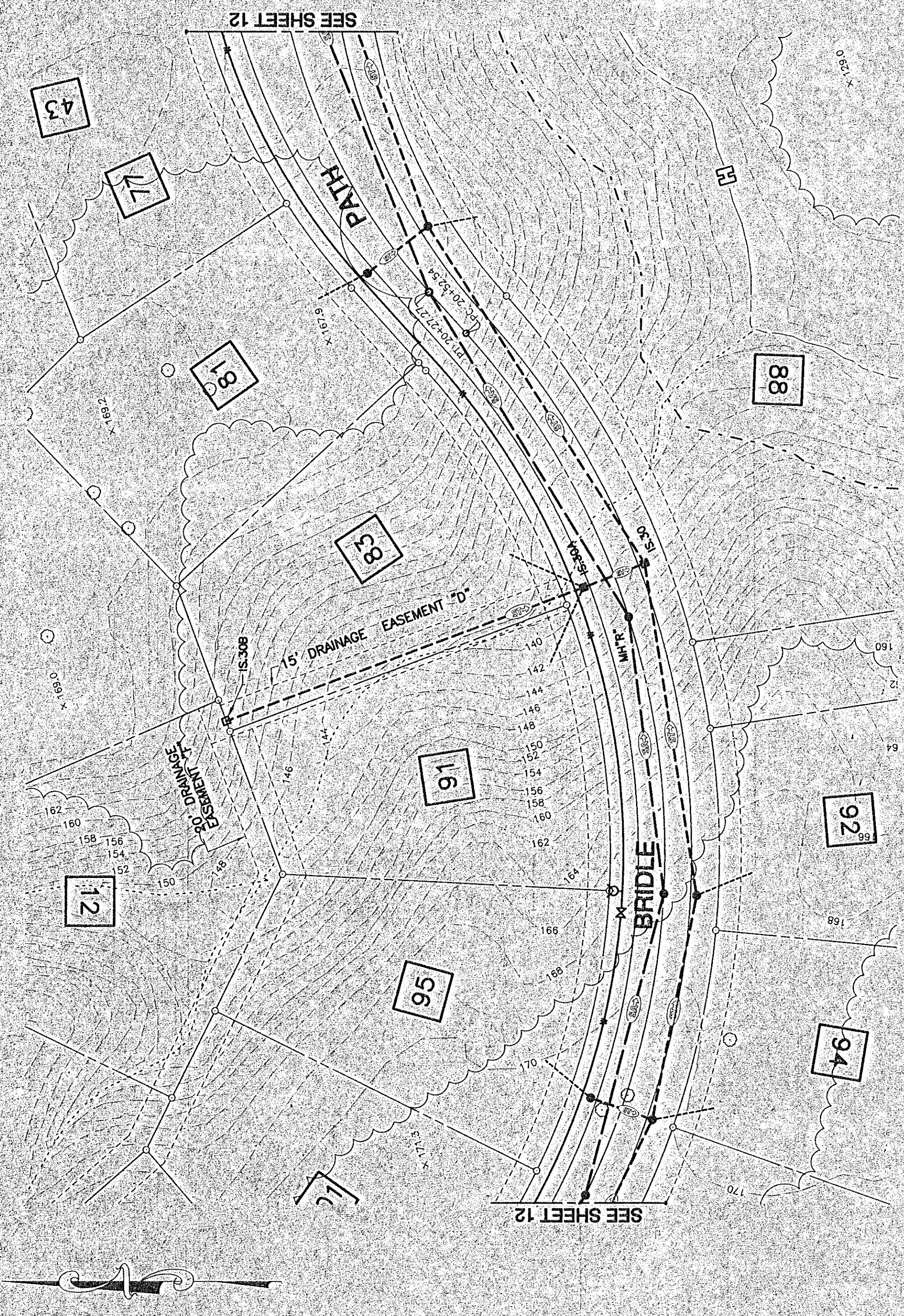
GENERAL PLAN - DRAINAGE EASEMENT "D" SCALE: 1" = 40'
