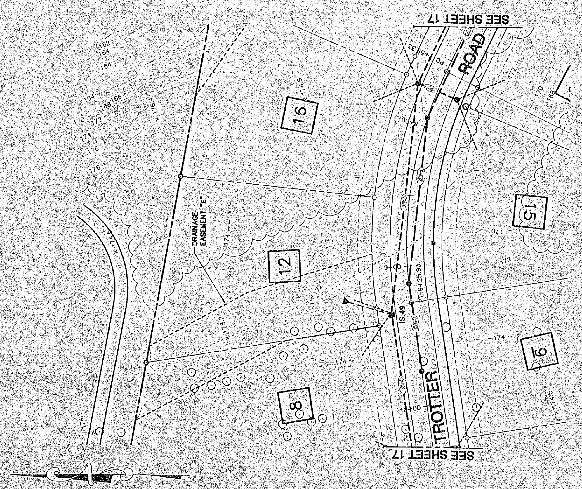
GENERAL PLAN - DRAINAGE EASEMENTS "E" SCALE: 1" = 40'
