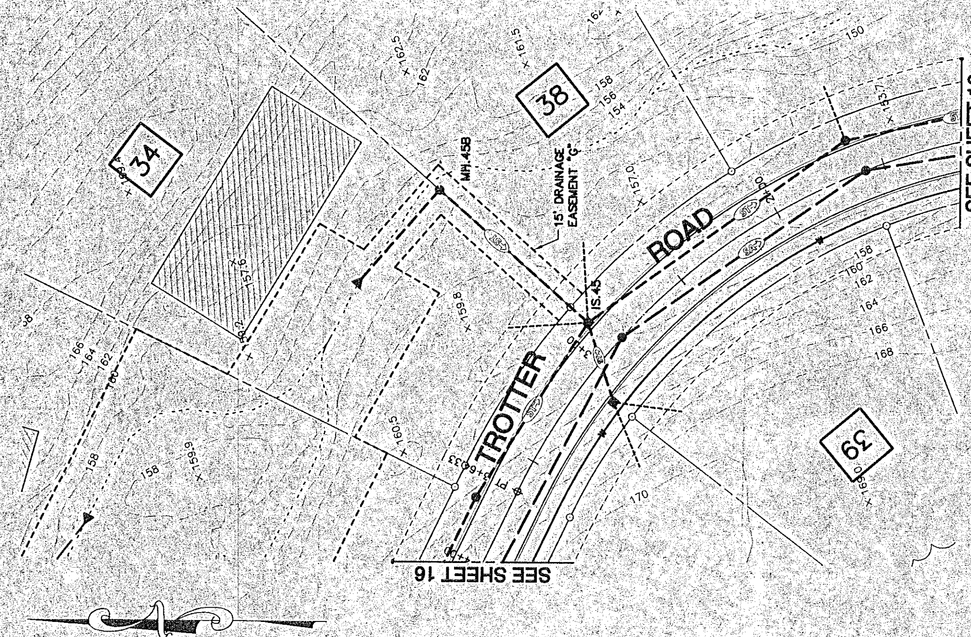
GENERAL PLAN - DRAINAGE EASEMENT "G" SCALE: 1" = 40'
