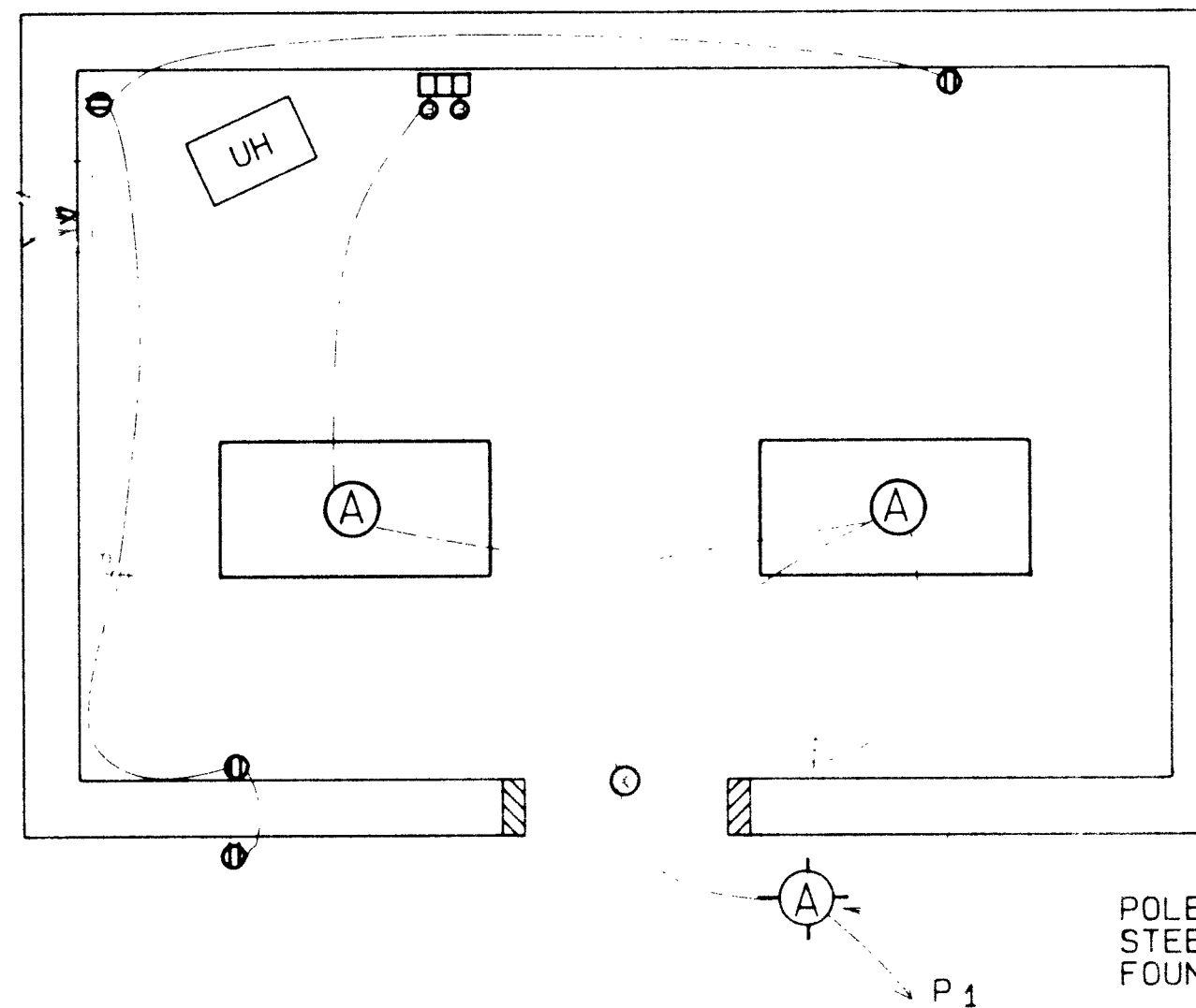
ELECTRICAL PLAN/GRADE FLOOR
