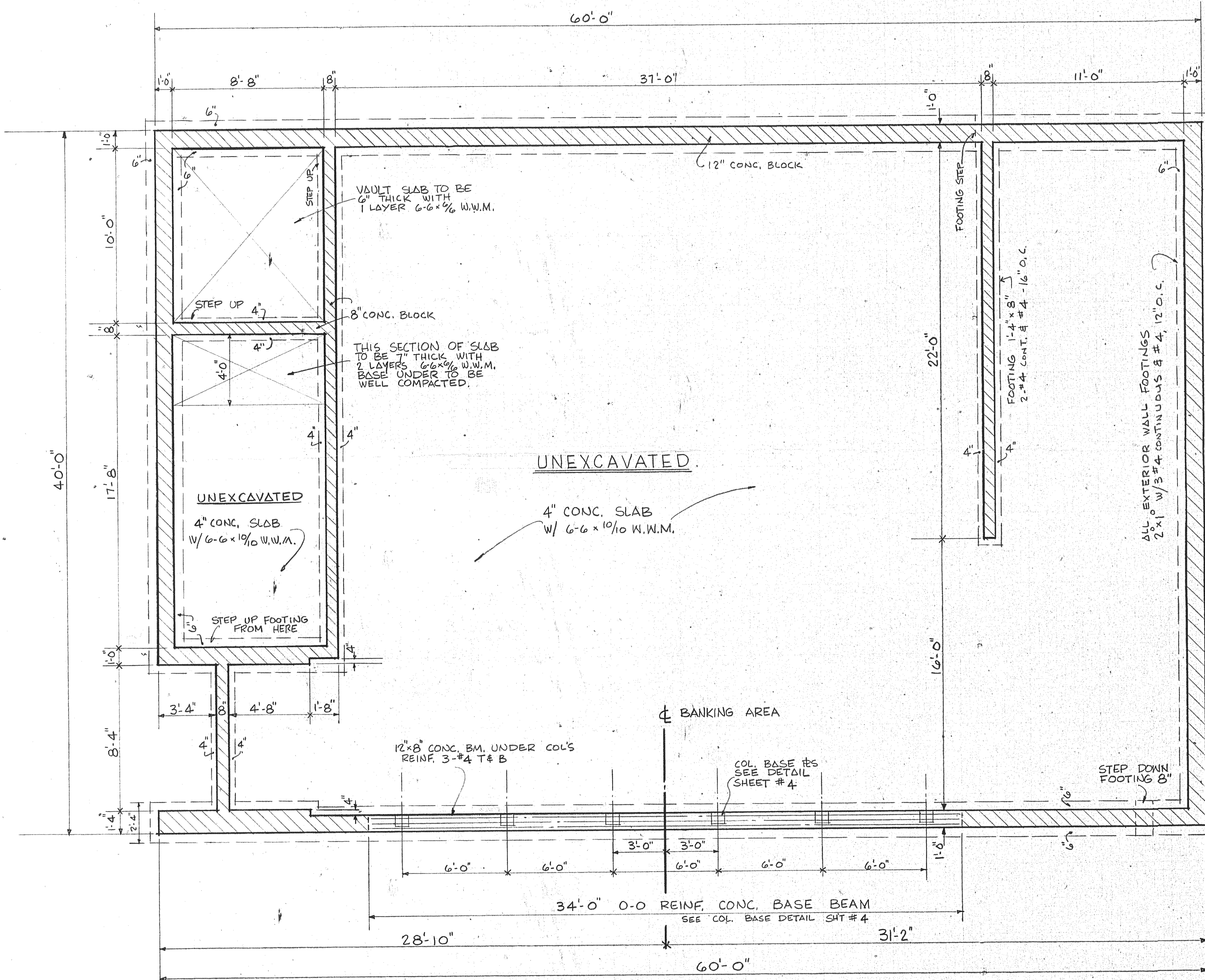
FOUNDATION PLAN — 1/4"=1'-0"
