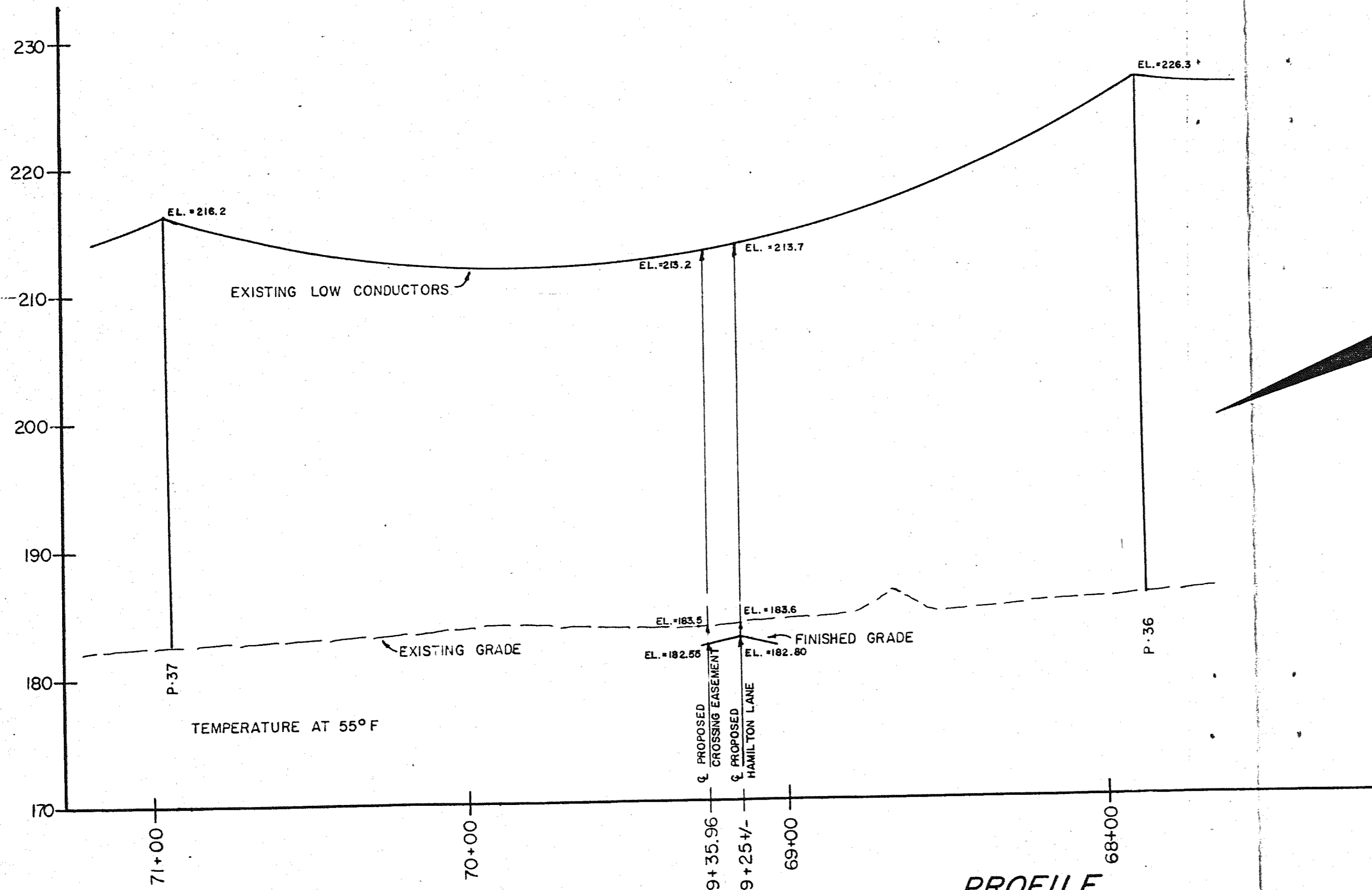
PROFILE SCALE: HORIZONTAL: 1" = 40' VERTICAL: 1" = 10'
