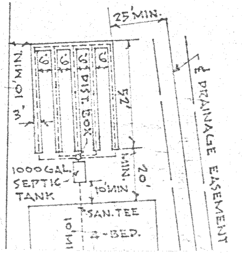
PLAN SCALE - 1"=50'
