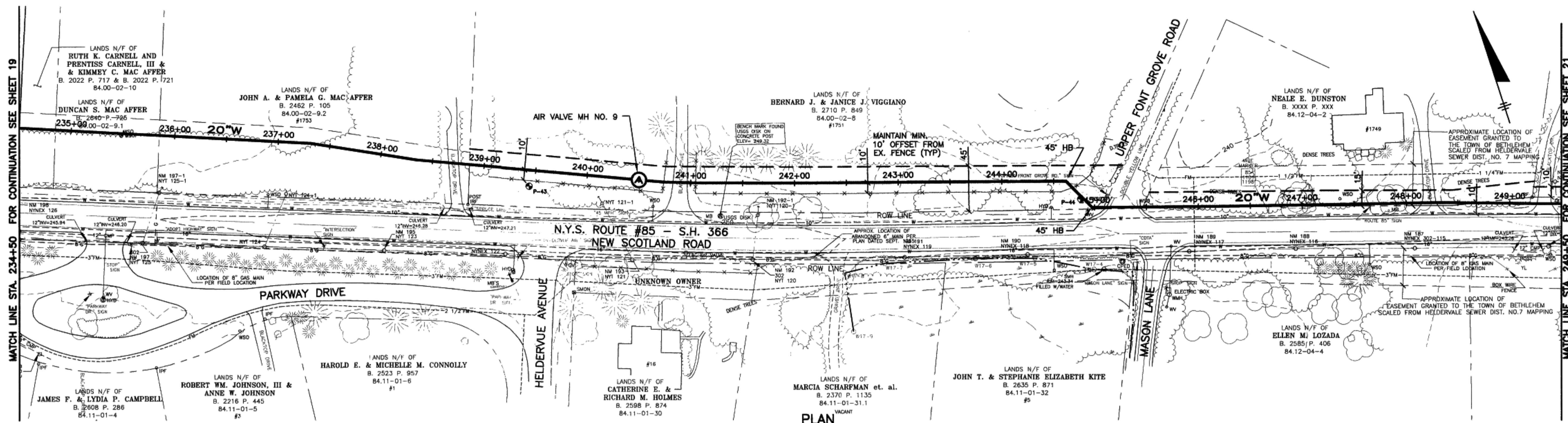
PLAN SCALE: 1"=50'
