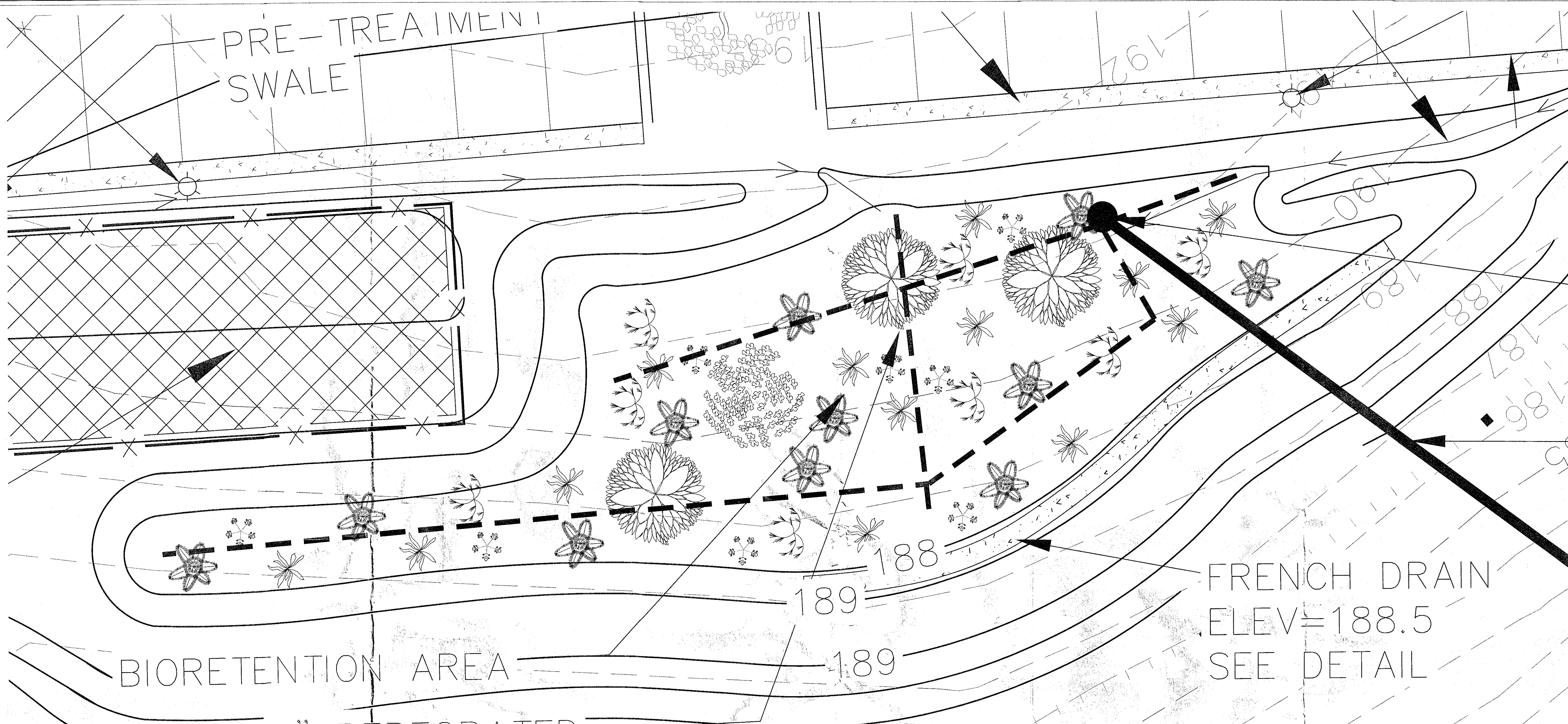
BIORETENTION AREA PLANTING DETAIL
