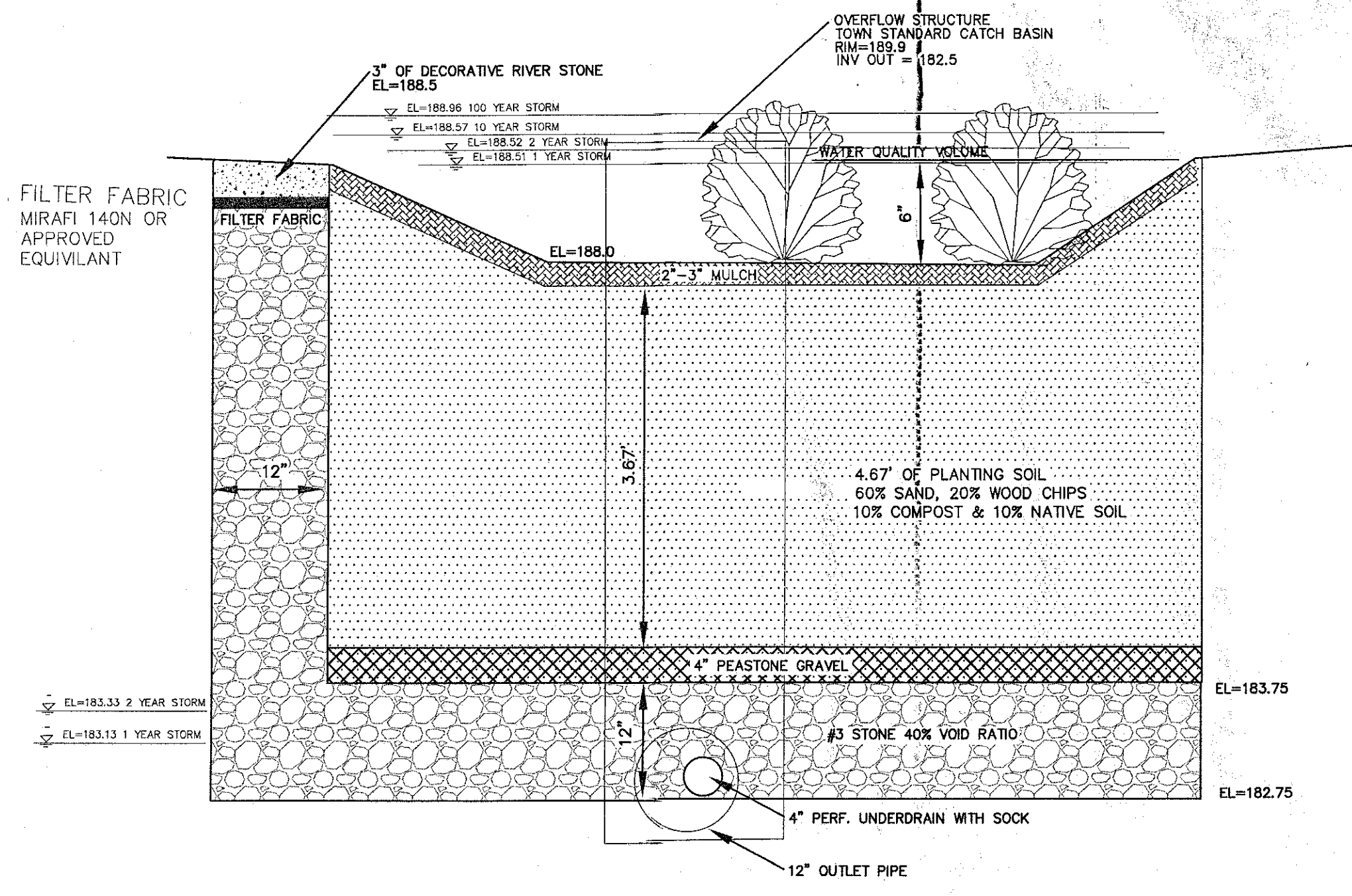
BIORETENTION AND STORAGE AREA
