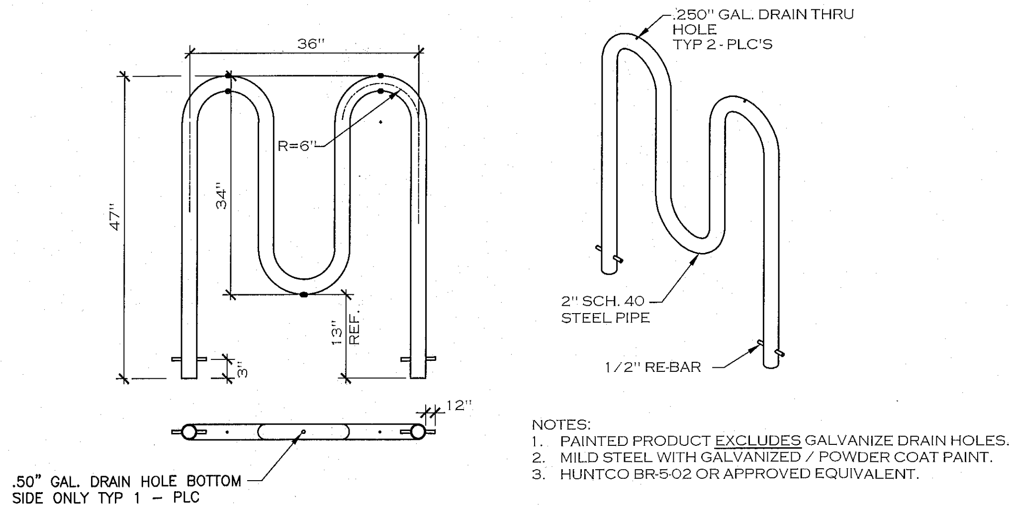
BIKE RACK DETAIL
