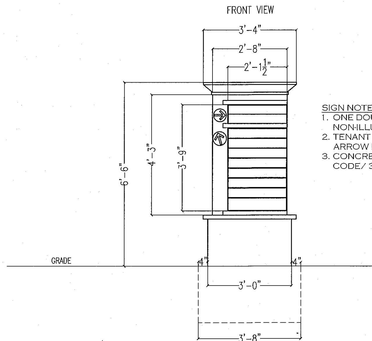
DIRECTIONAL SIGN DETAIL
