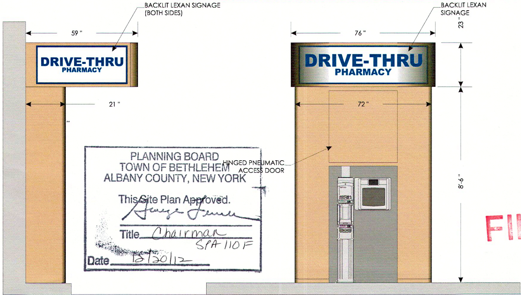
APPROACH ELEVATION
