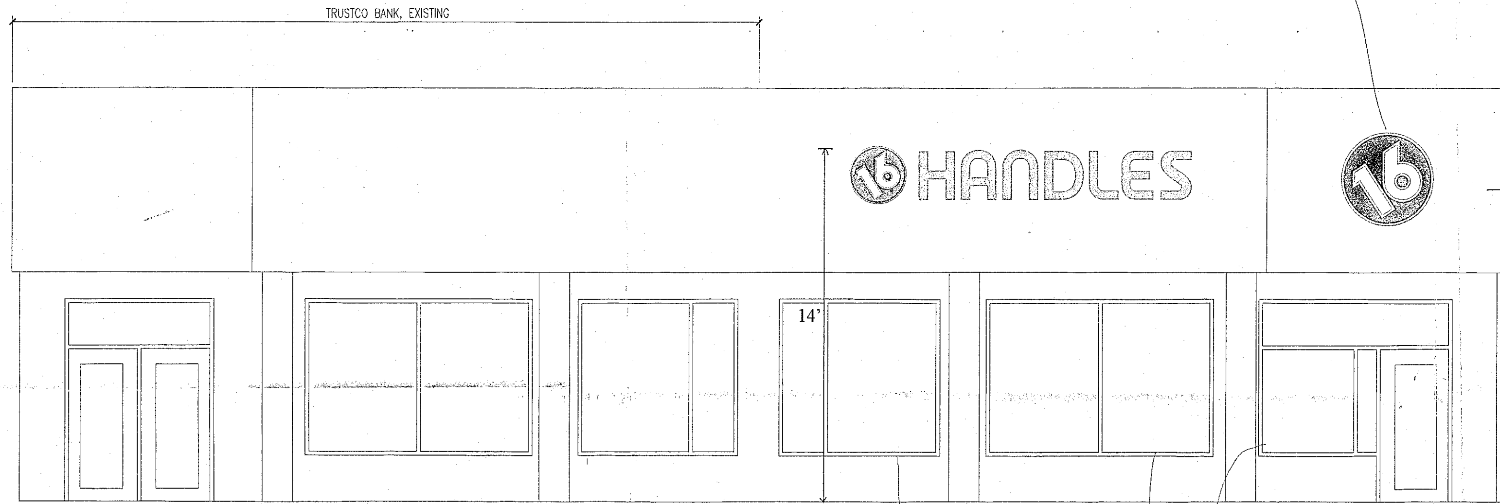
2 PROPOSED ELEVATION 1/4"=1'-0"
