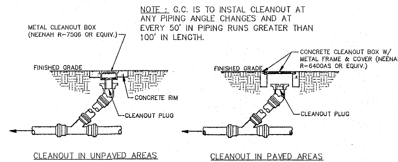
EXTERIOR CLEANOUT DETAILS
