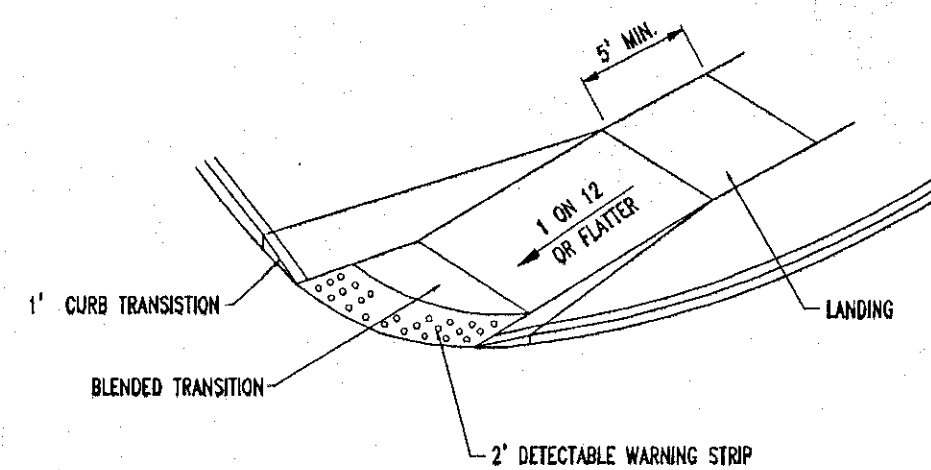
NYS DOT R.O.W. SIDEWALK CURB RAMP/BLENDED TRANSITION
