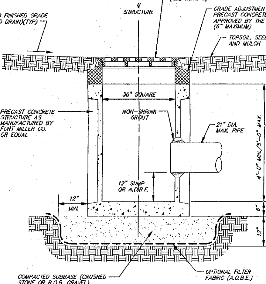
PRECAST CONCRETE CATCH BASIN
