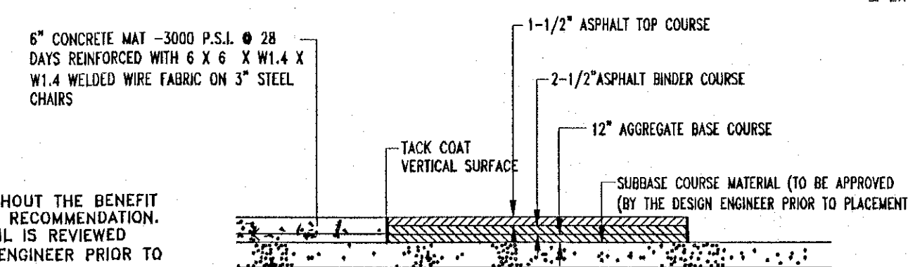
CONCRETE & BITUMINOUS CONCRETE PAVING DETAIL
