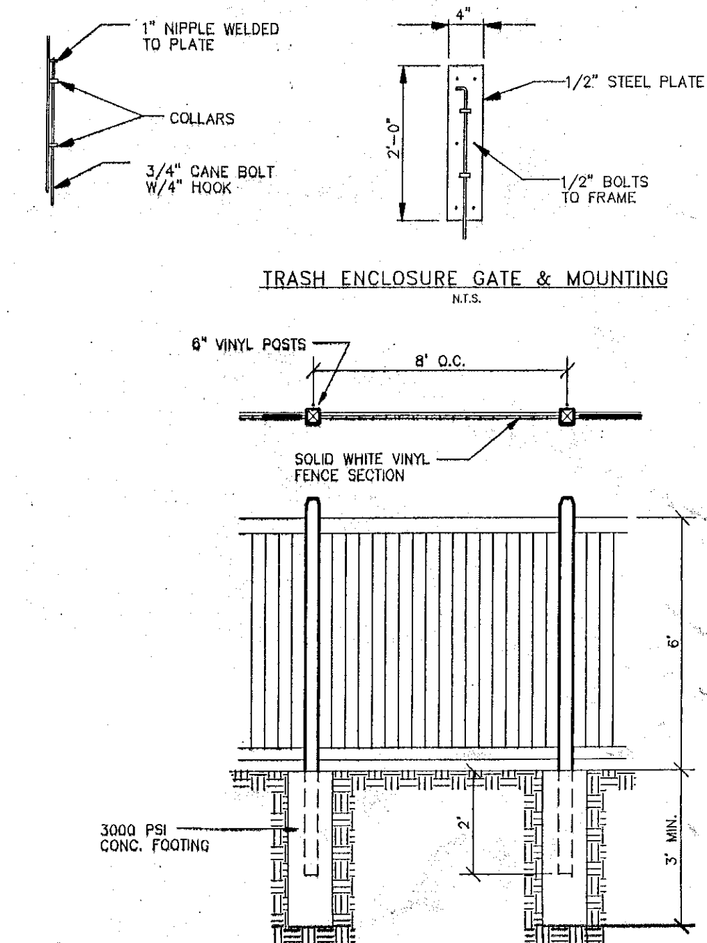
VINYL FENCE DETAIL
