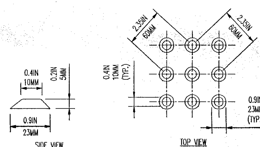
DETECTABLE WARNING STRIP DETAIL
