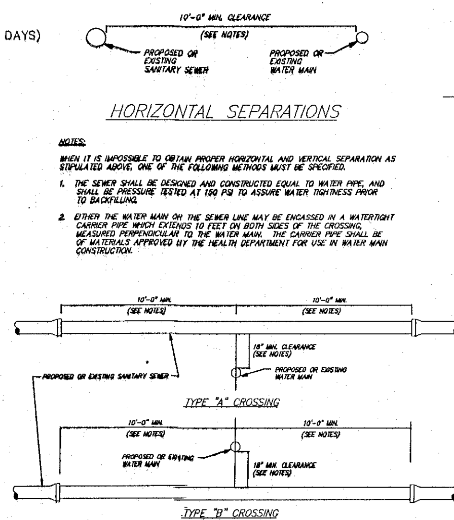
SEWER MAIN AND WATER MAIN SEPERATION SCALE: N.T.S.
