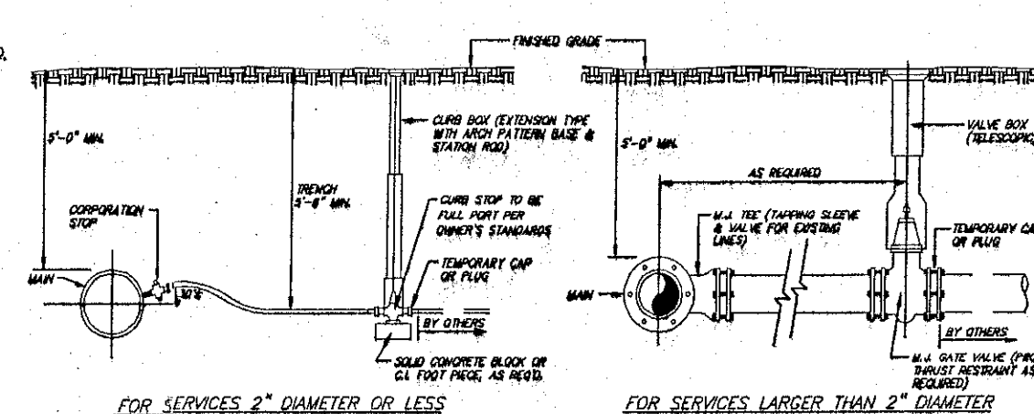
TYPICAL SERVICE CONNECTION DETAILS SCALE : NONE
