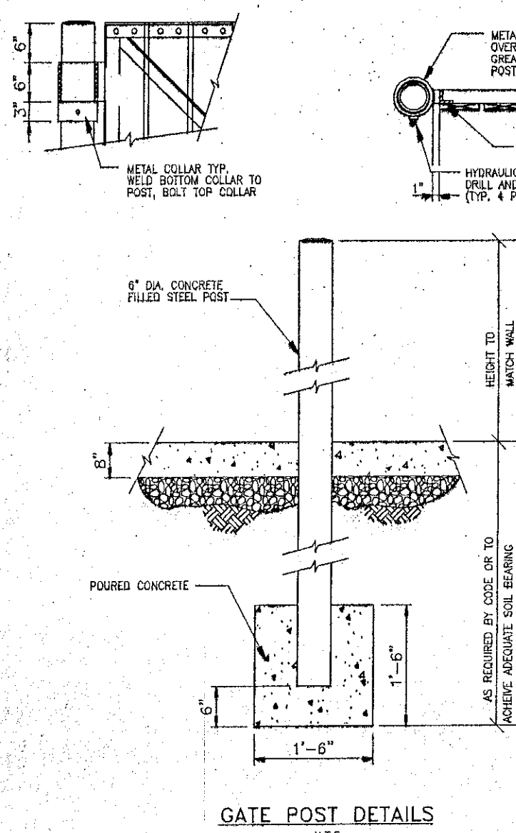
GATE POST DETAILS
