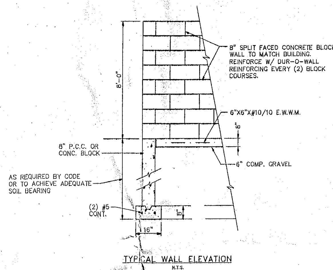
TYPICAL WALL ELEVATION N.T.S.
