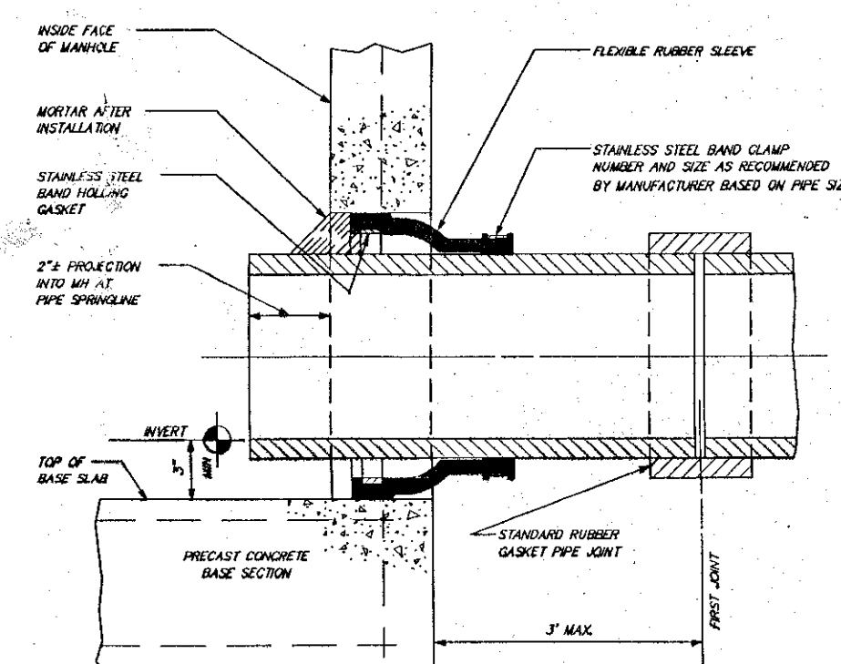
CORED OR PRECAST HOLE FLEXIBLE PIPE - TO - M.H. - JOINT
