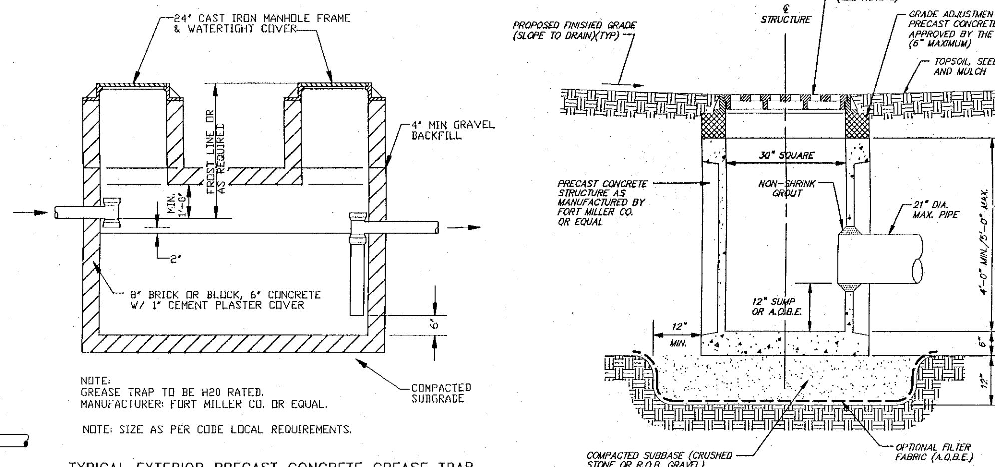
TYPICAL EXTERIOR PRECAST CONCRETE GREASE TRAP
