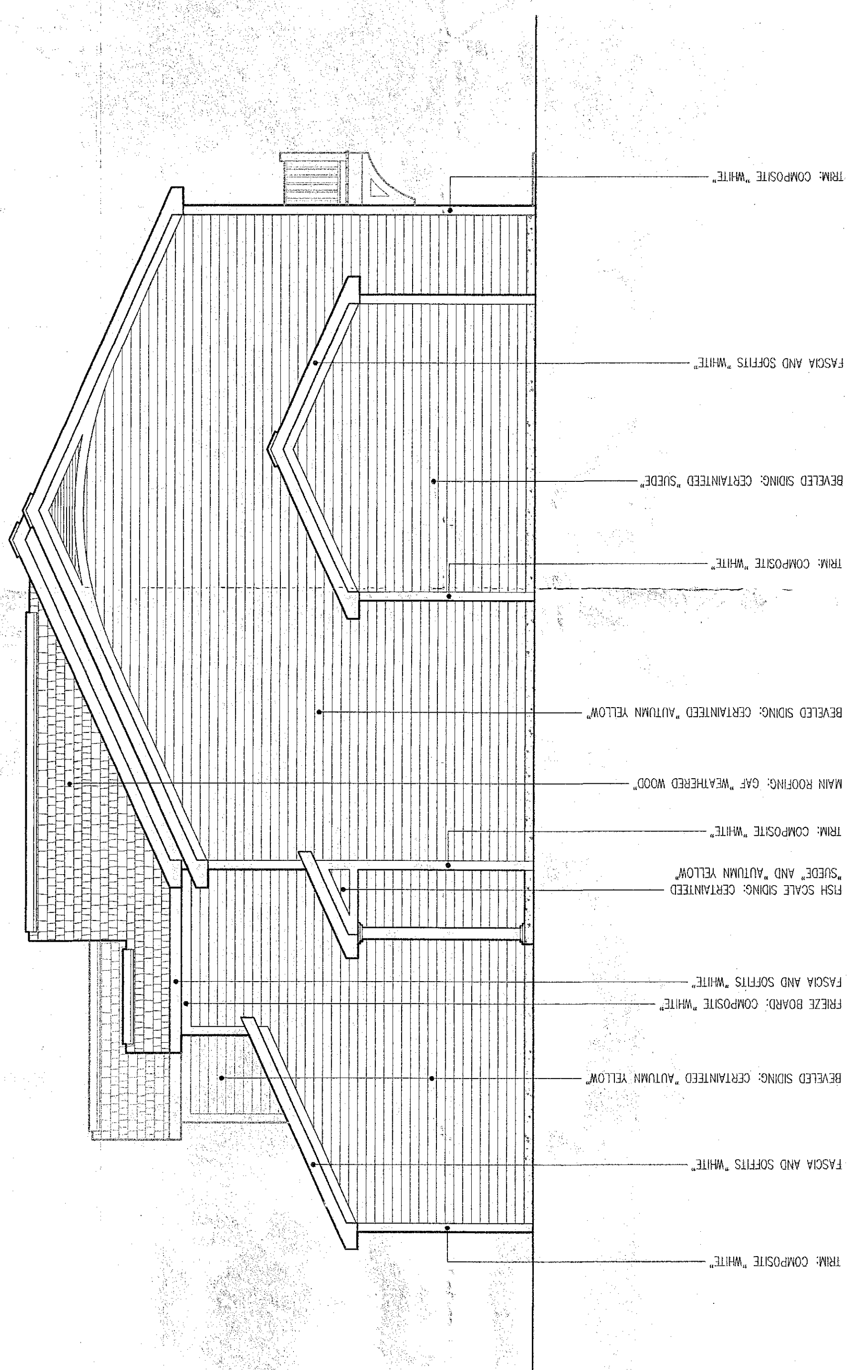
2 TYPICAL RIGHT SIDE ELEVATION
