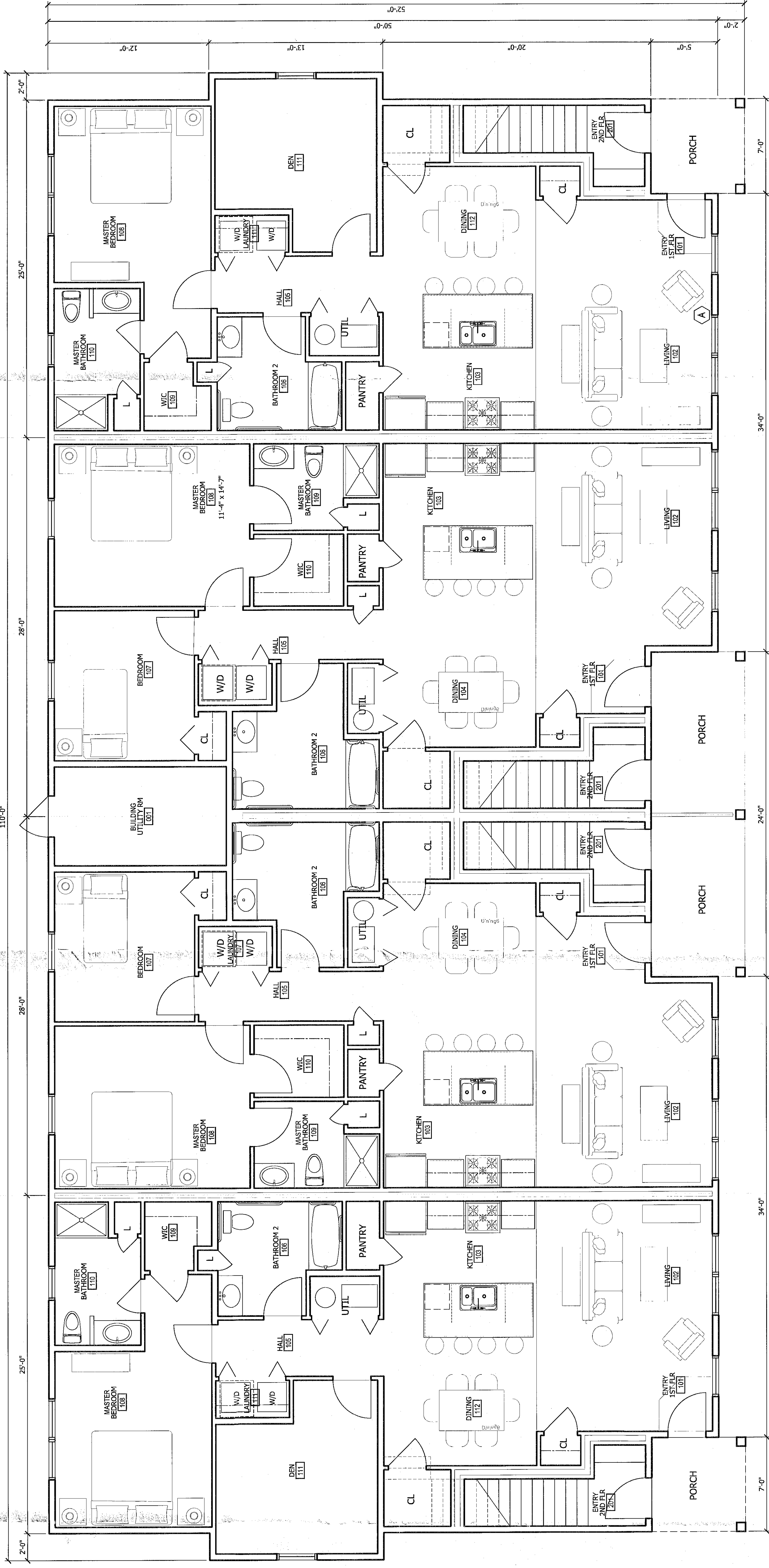
1st FLOOR PLAN - 8 UNIT
