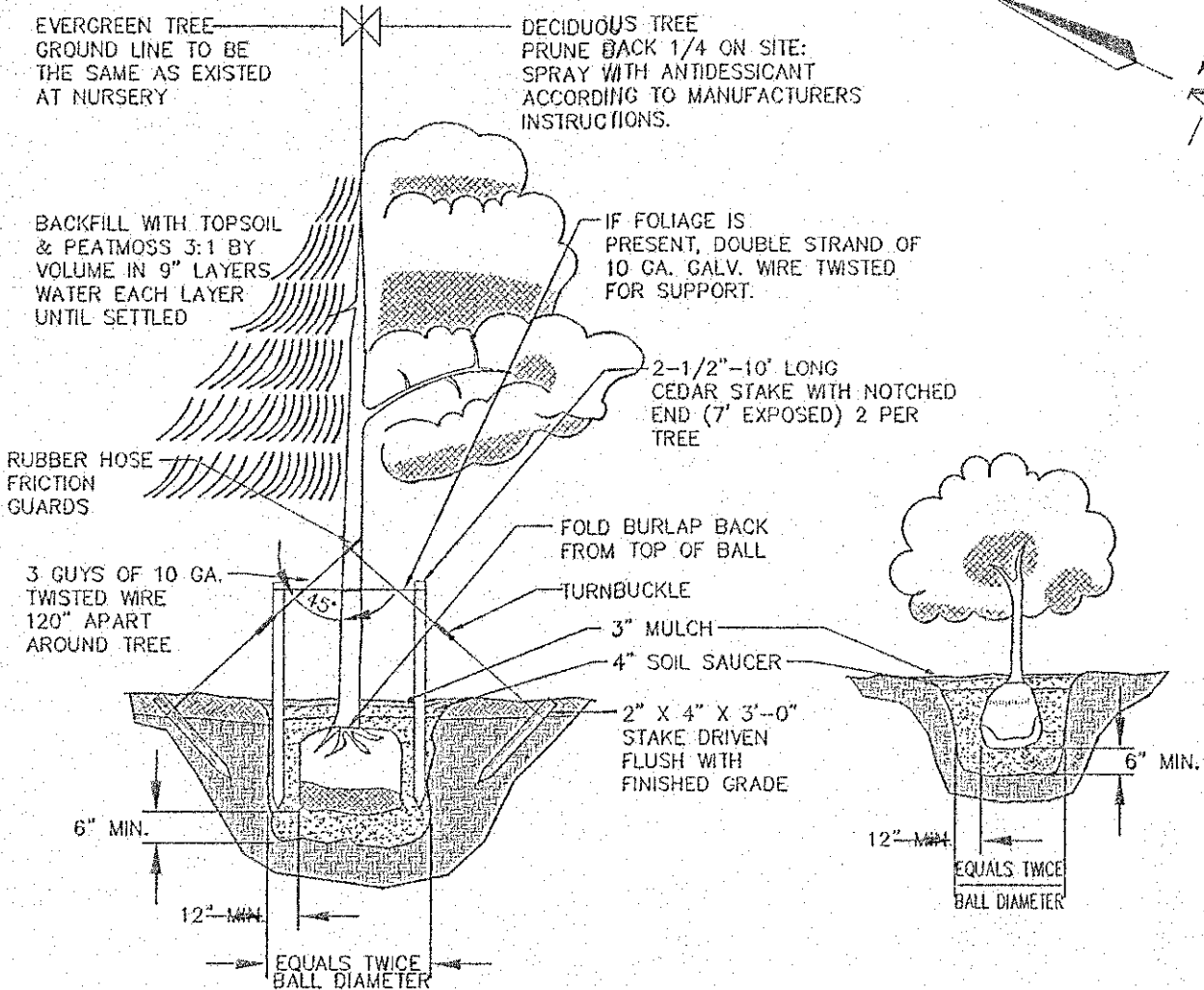
TYPICAL PLANTING DETAIL NOT TO SCALE
