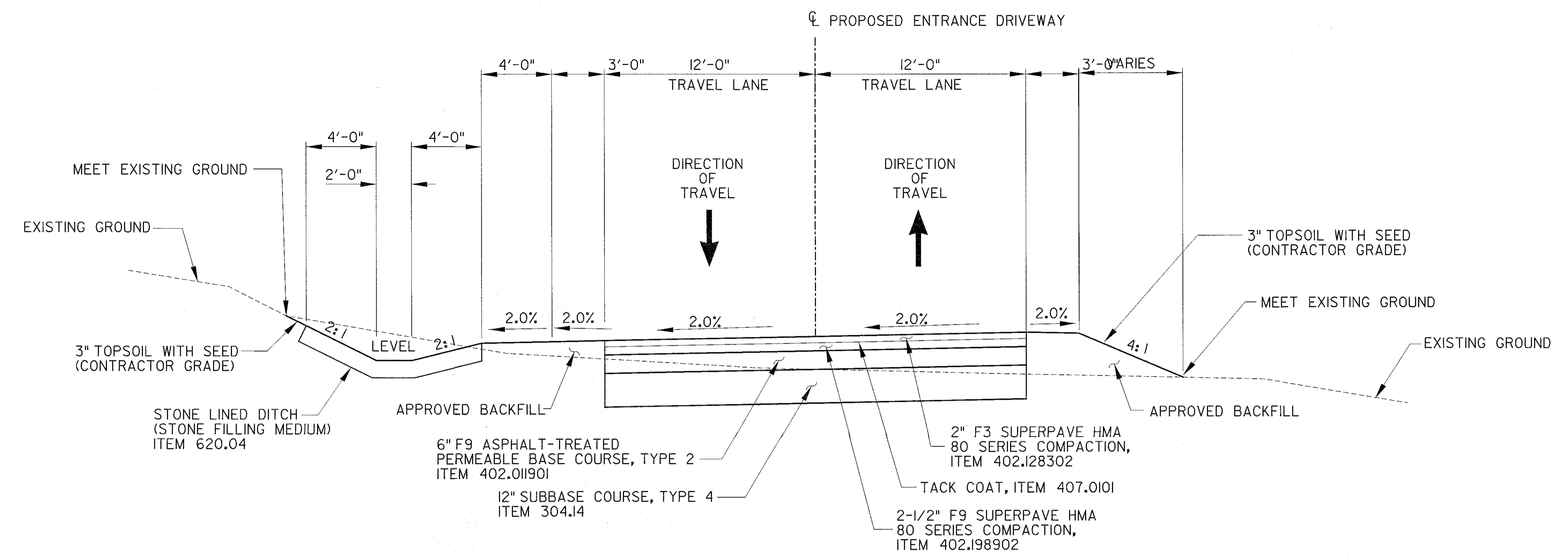
TYPICAL SECTION - ENTRANCE DRIVEWAY (LOOKING WEST) STA. A 10+12.00 TO STA. A 10+36.00 (APPROX.) NOT TO SCALE
