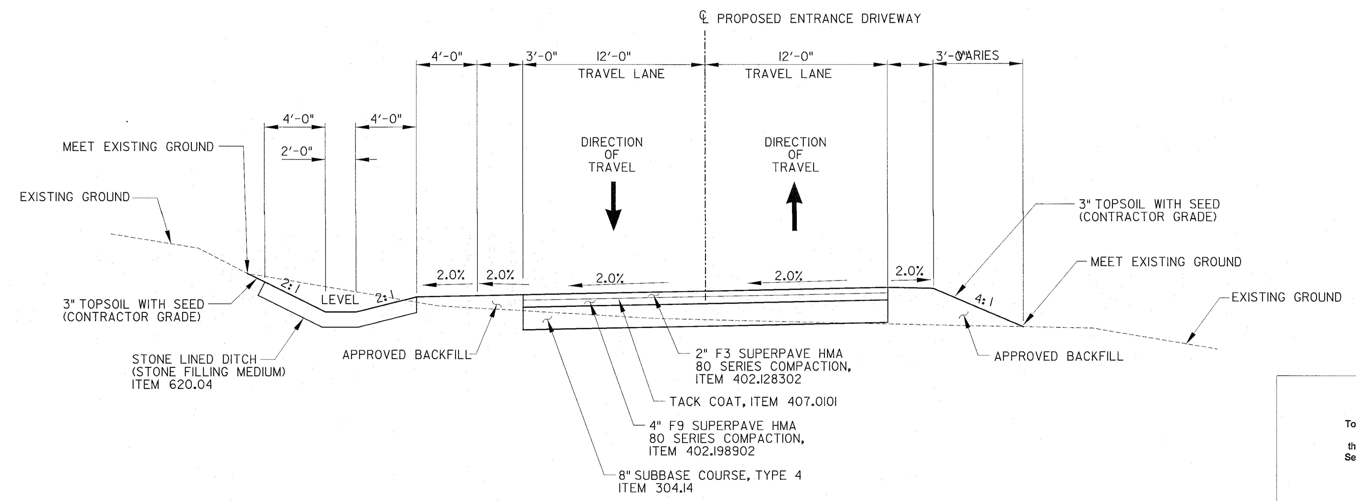
TYPICAL SECTION - ENTRANCE DRIVEWAY (LOOKING WEST) STA. A 10+36.00 TO STA. A 11+93.75 NOT TO SCALE
