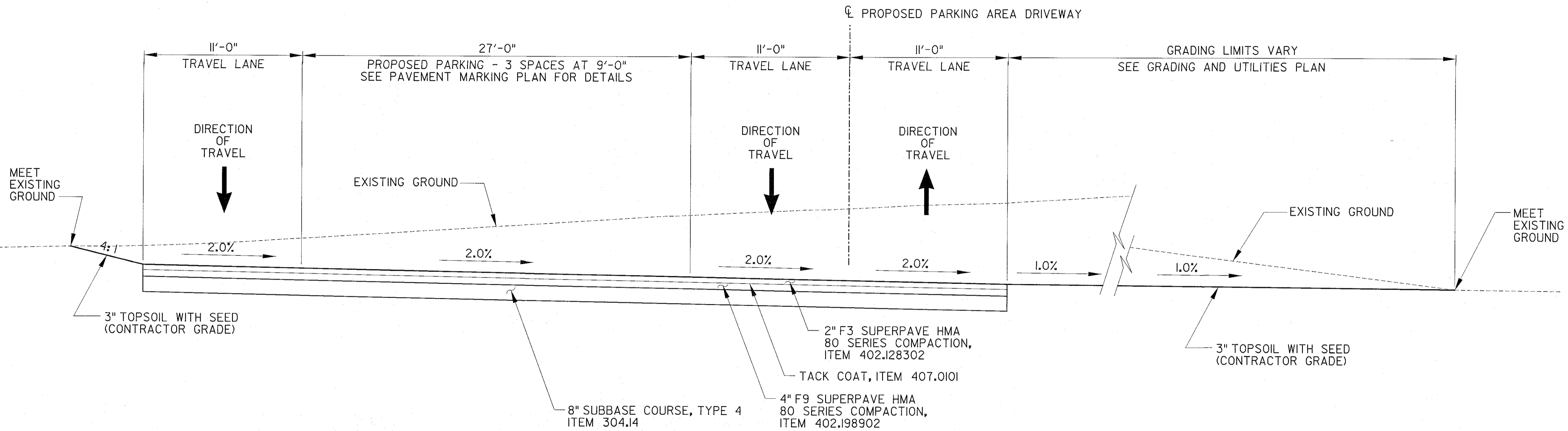
TYPICAL SECTION - PARKING AREA (LOOKING NORTH) NOT TO SCALE
