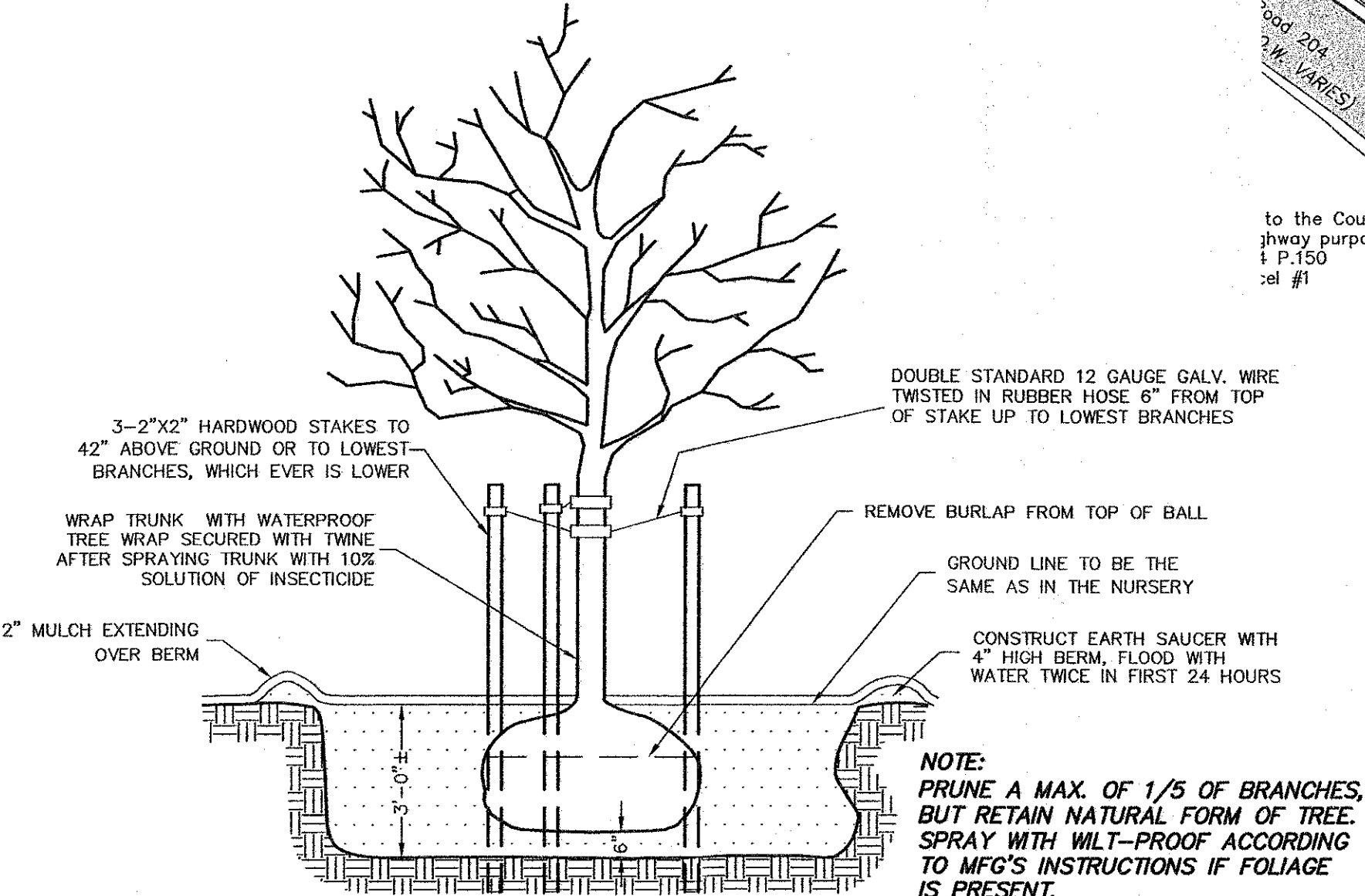
NEW TREE PLANTING DETAIL NOT TO SCALE
