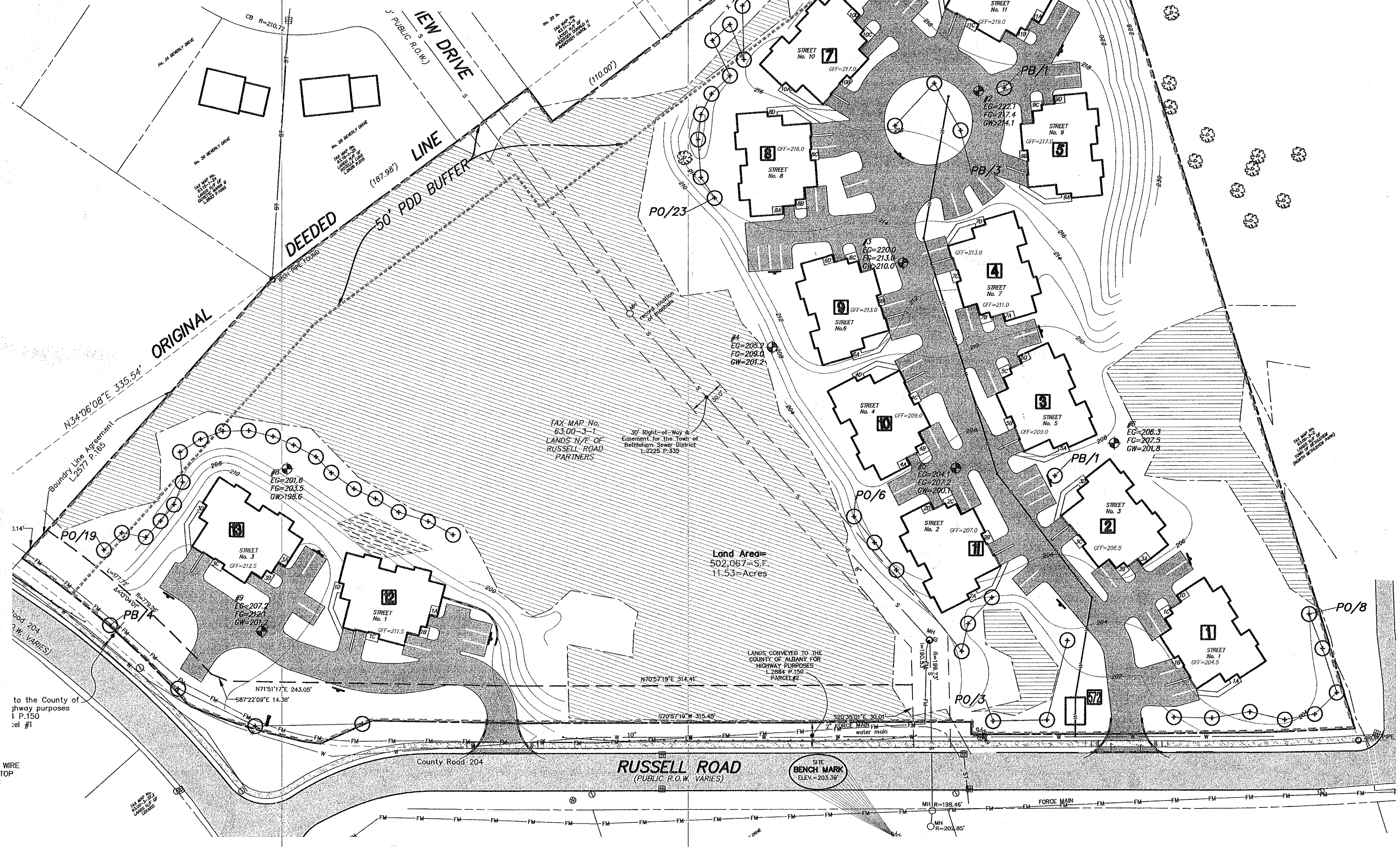
OVERALL LANDSCAPE PLAN SCALE 1"=20'
