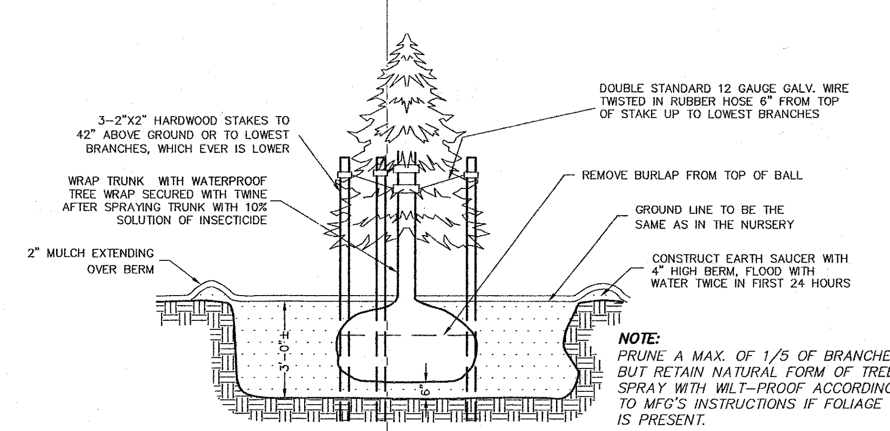
NEW EVERGREEN TREE PLANTING DETAIL NOT TO SCALE
