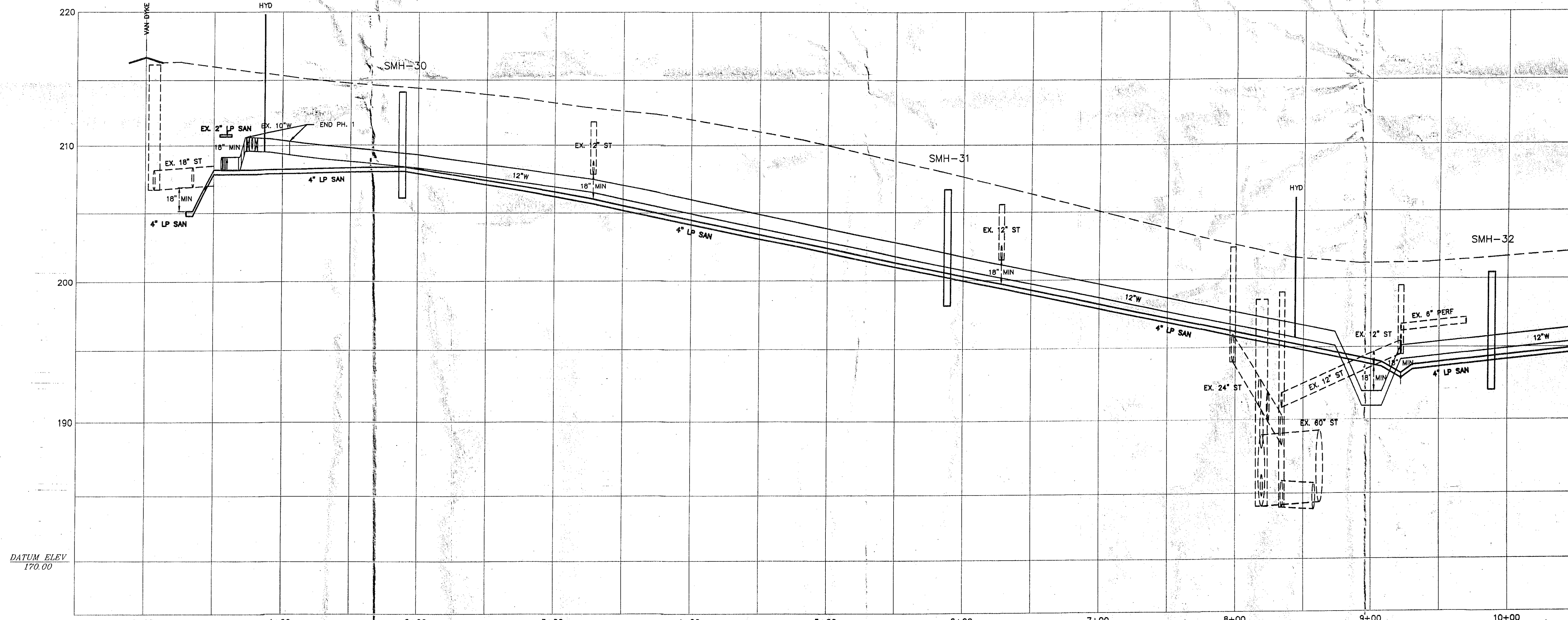
PROFILE OF DELMAR BYPASS [STA 0+00 THRU 10+50]
