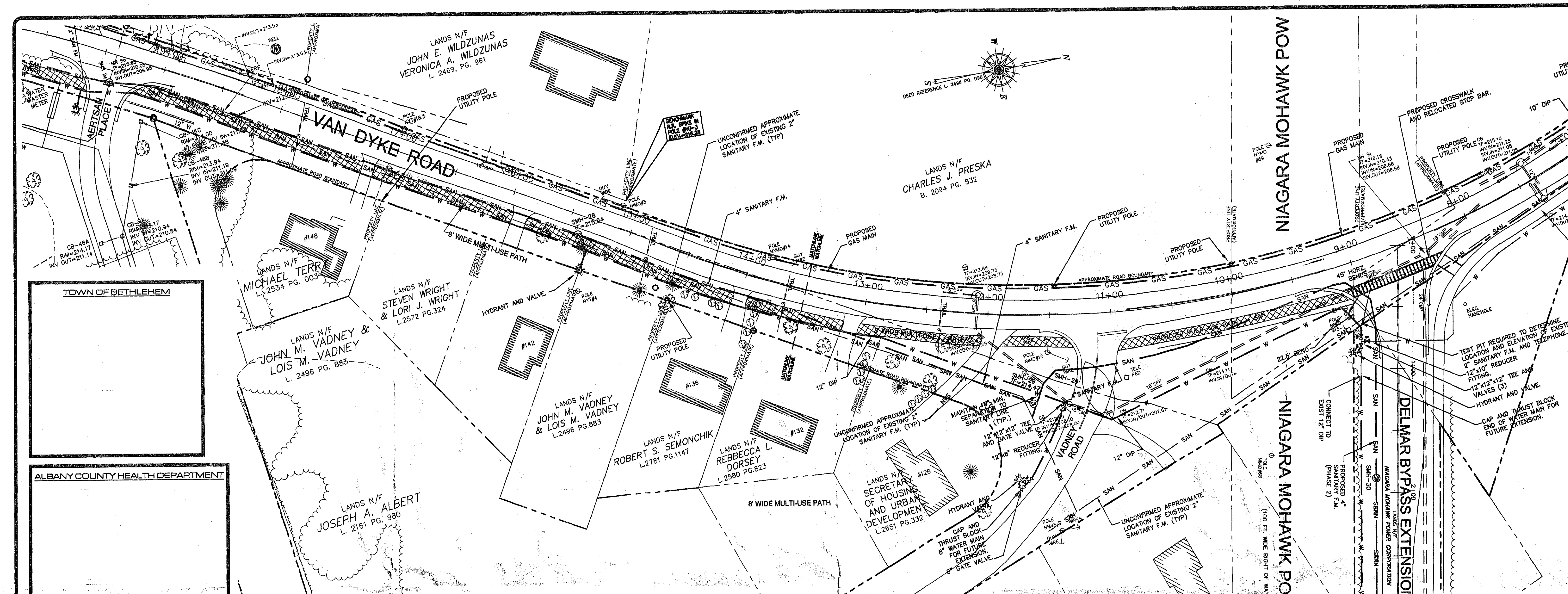
PLAN OF VAN DYKE ROAD (STA 19+50 THRU 8+50) SCALE: (1"=40')
