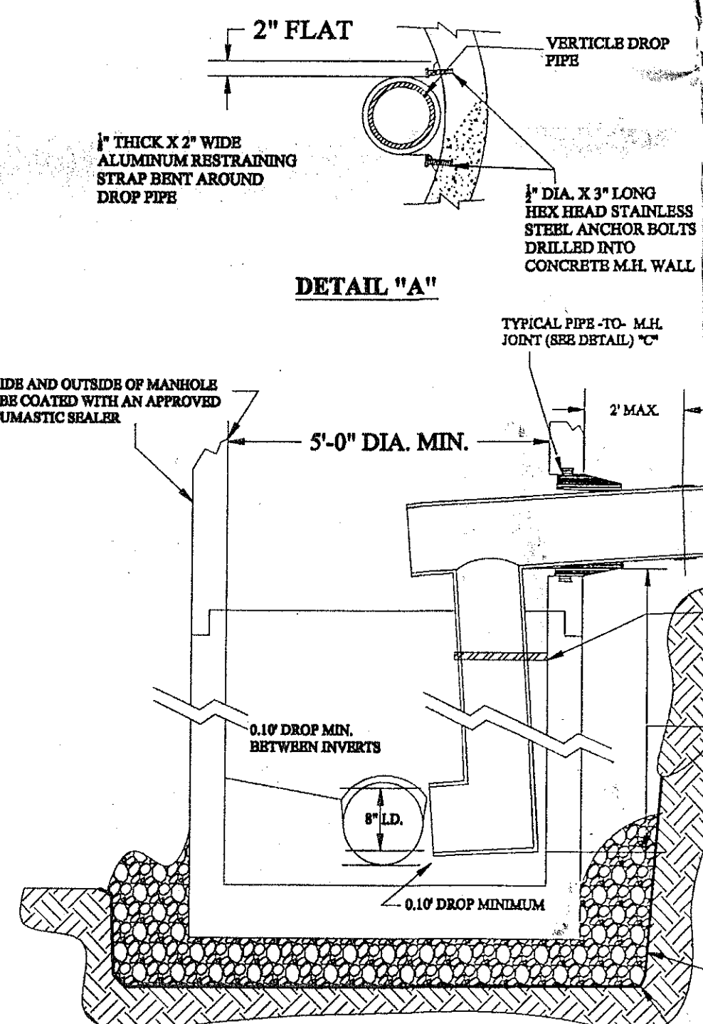
DROP MAN HOLE DETAIL
