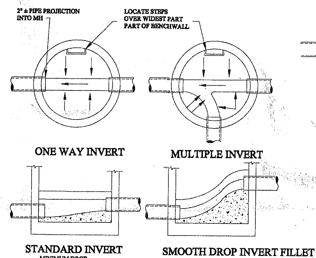
INVERT CHANNEL AND BENCHWALL DETAIL "D"
