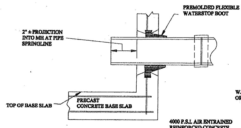
FLEXIBLE PIPE - TO - M.H. JOINT DETAIL "C"
