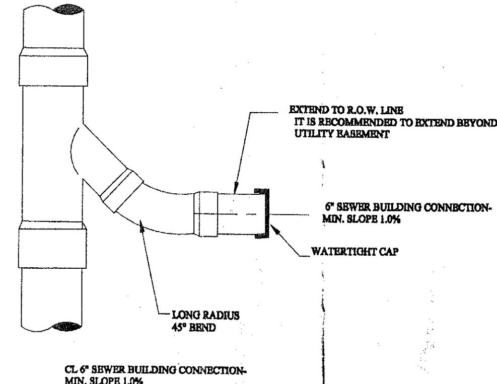
WYE SEWER BUILDING CONNECTION
