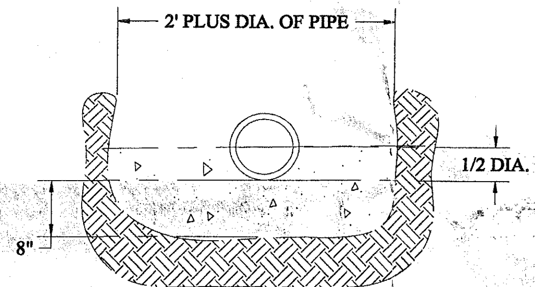
CONCRETE CRADLE FOR PIPE
