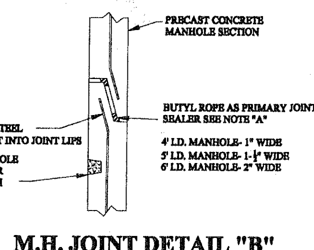
M.H. JOINT DETAIL "B"
