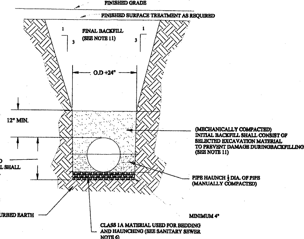
BEDDING DETAIL
