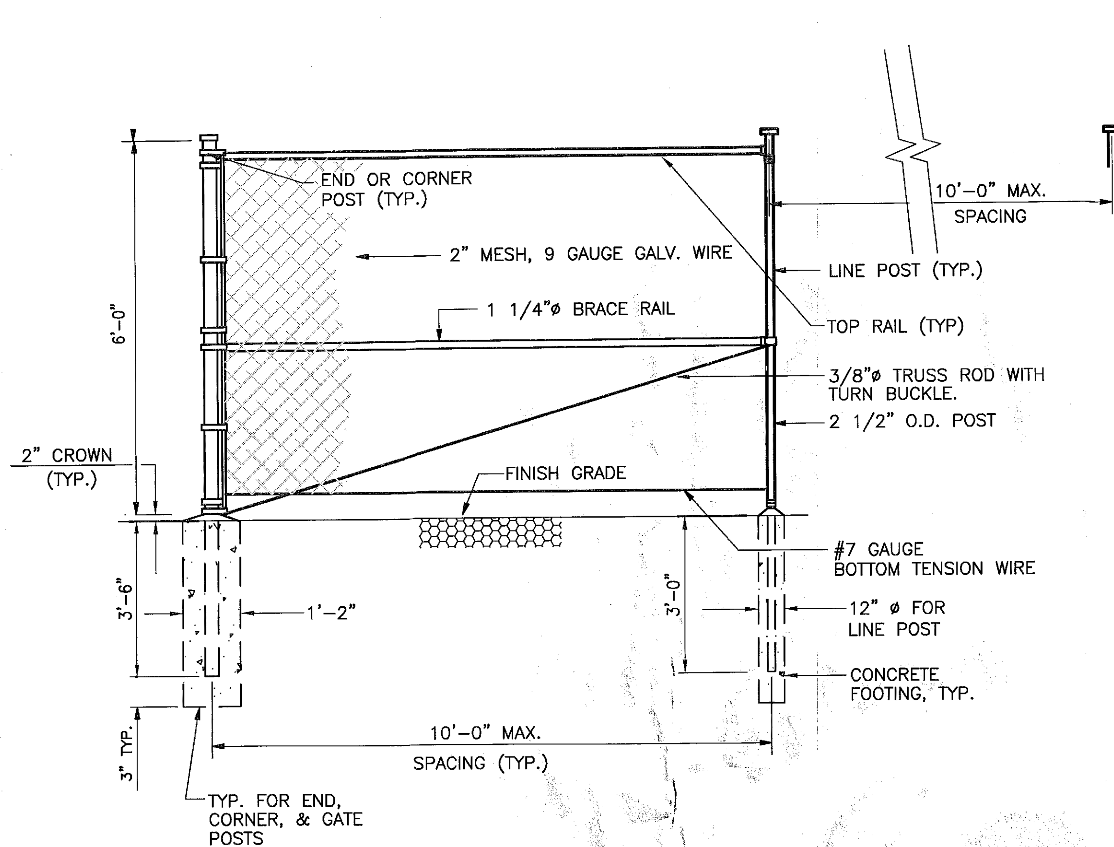
1 CHAIN LINK FENCE DETAIL (ELEVATION) NOT TO SCALE
