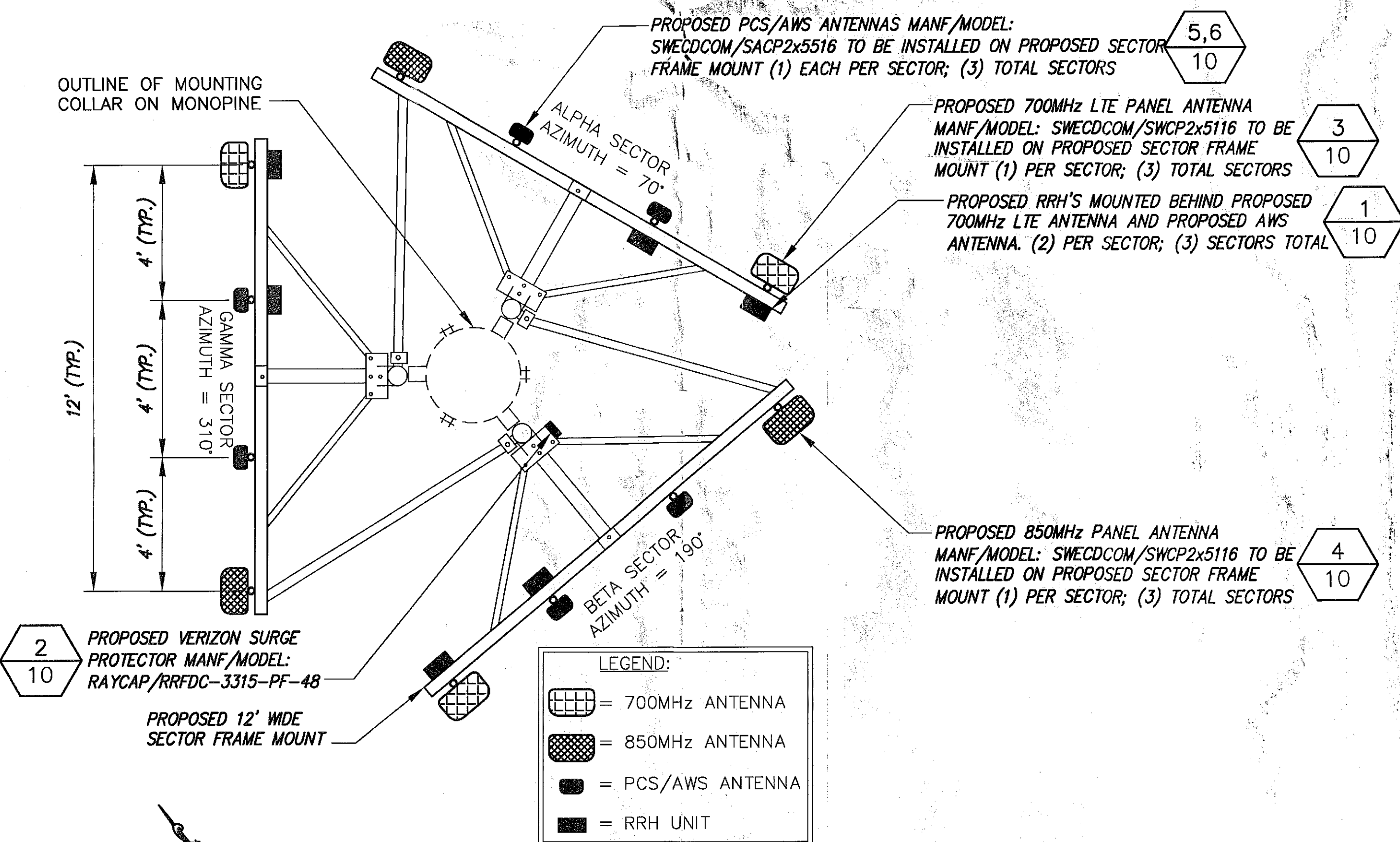
3 VERIZON ANTENNA AND RRH CONFIGURATION NOT TO SCALE
