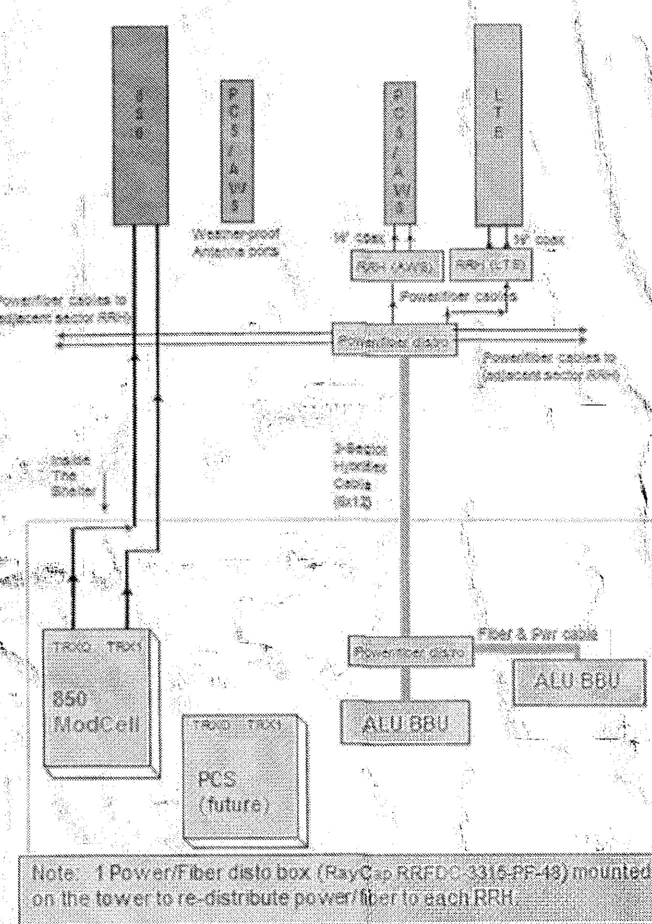
1 VERIZON WIRELESS PROPOSED ALPHA COAX DIAGRAM NOT TO SCALE
