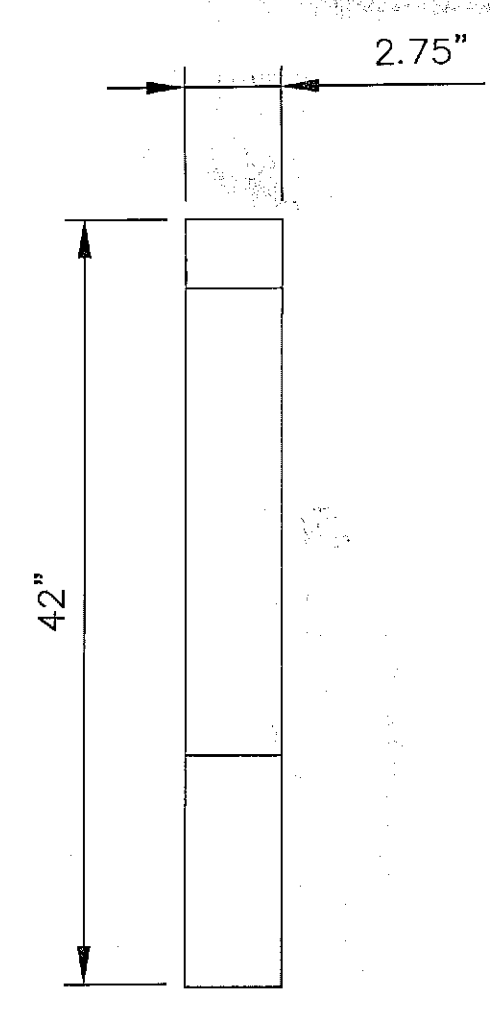
ELEVATION PLAN
