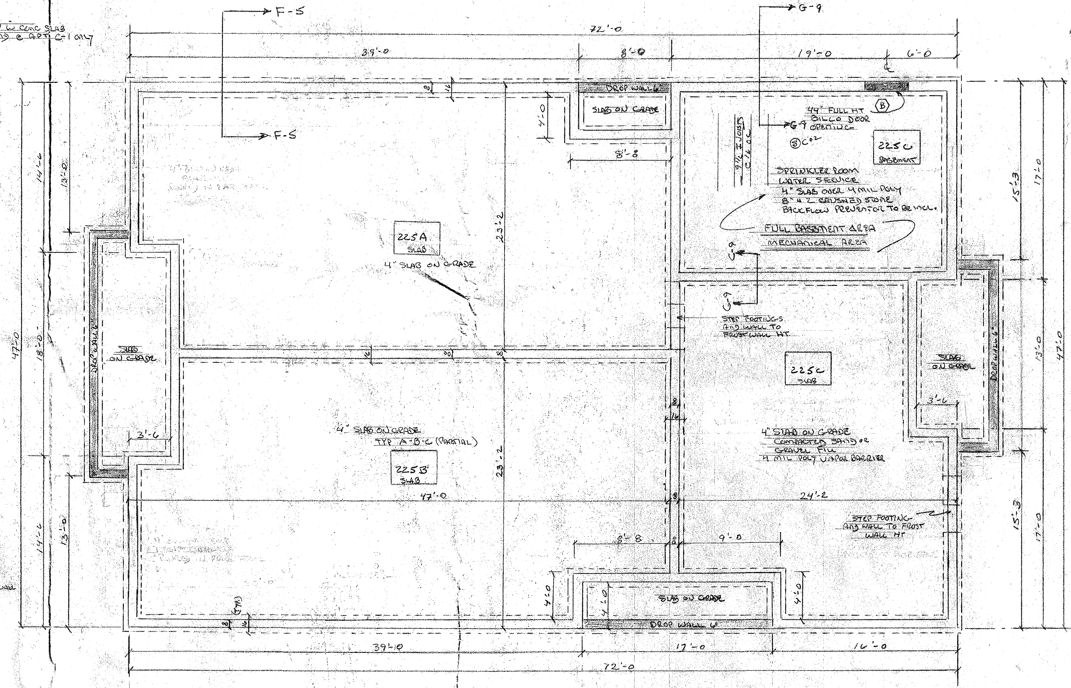
FOUNDATION PLAN 1/4" = 1'-0"
