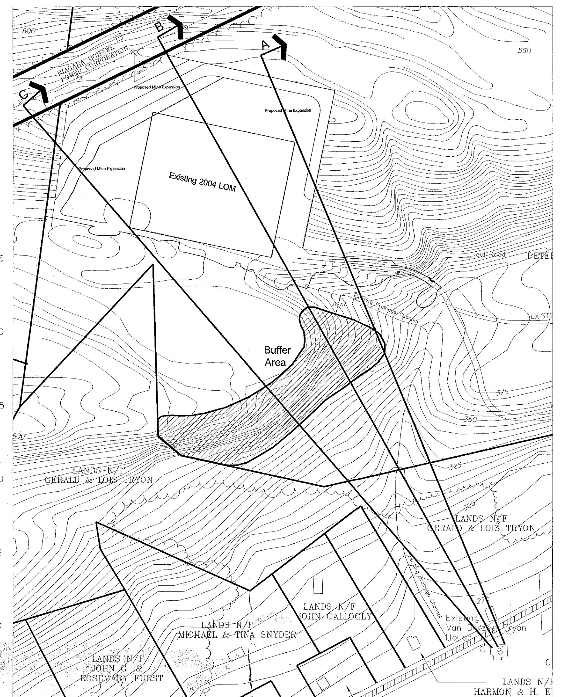
Section Plan
