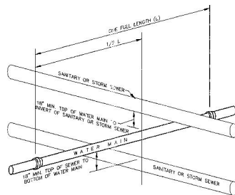
1 TYPICAL SECTION WATER / SEWER CROSSING SCALE: NONE CROSS REFERENCE: NONE
