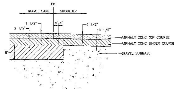
4 NYS ROUTE 9W SHOULDER PAVEMENT TRANSITION SCALE: NONE CROSS REFERENCE: NONE
