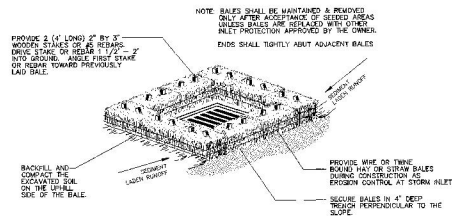
2 INLET PROTECTION SCALE: NONE CROSS REFERENCE: NONE
