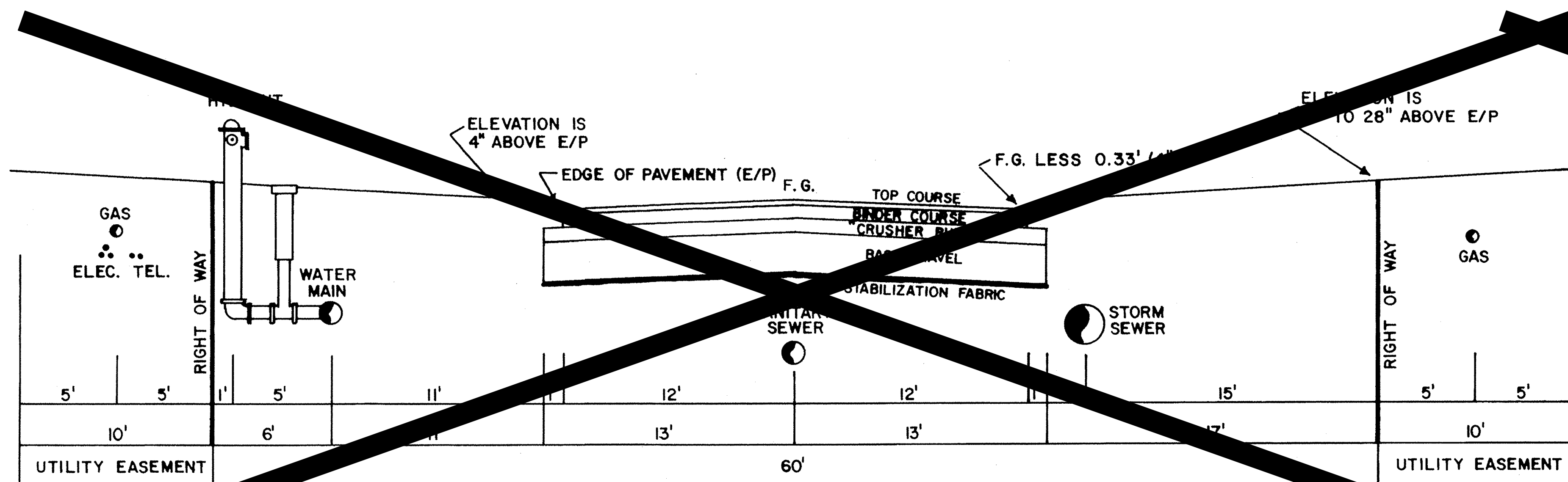
TYPICAL 60' RIGHT OF WAY
