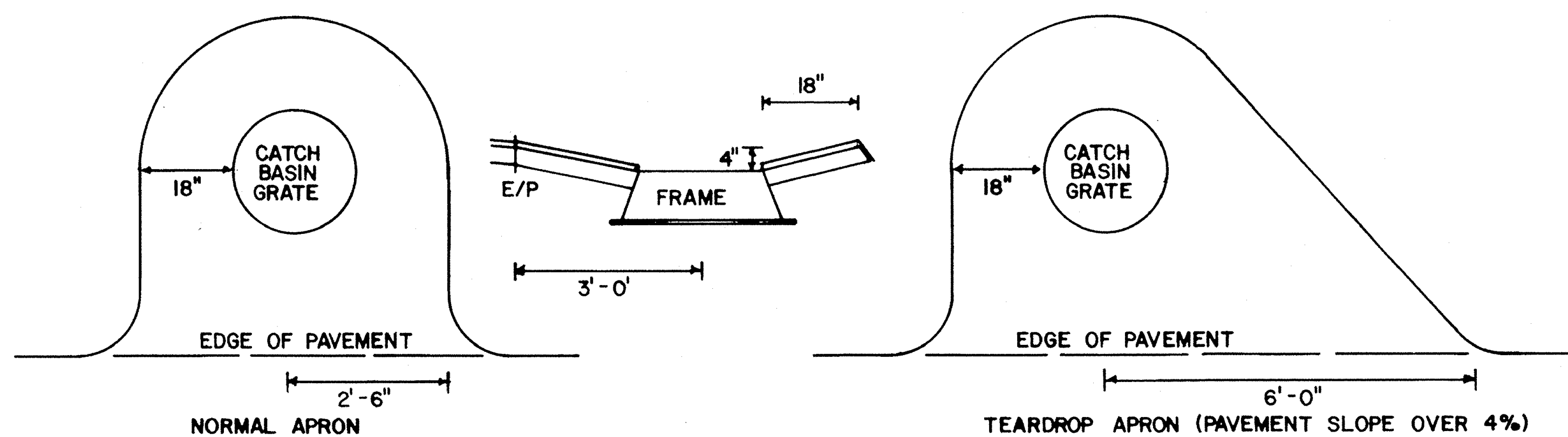
TYPICAL CATCH BASIN APRONS
