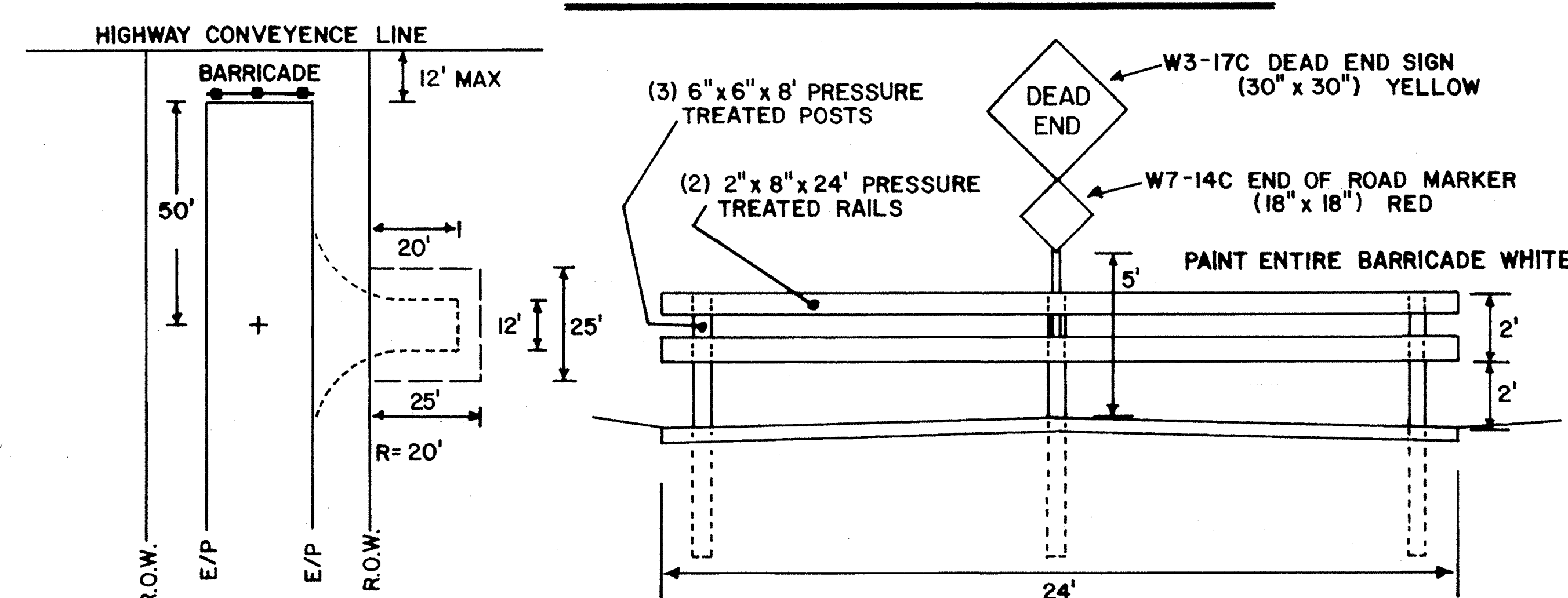
TYPICAL DEAD END, TEMPORARY TURN AROUND AND BARRICADE
