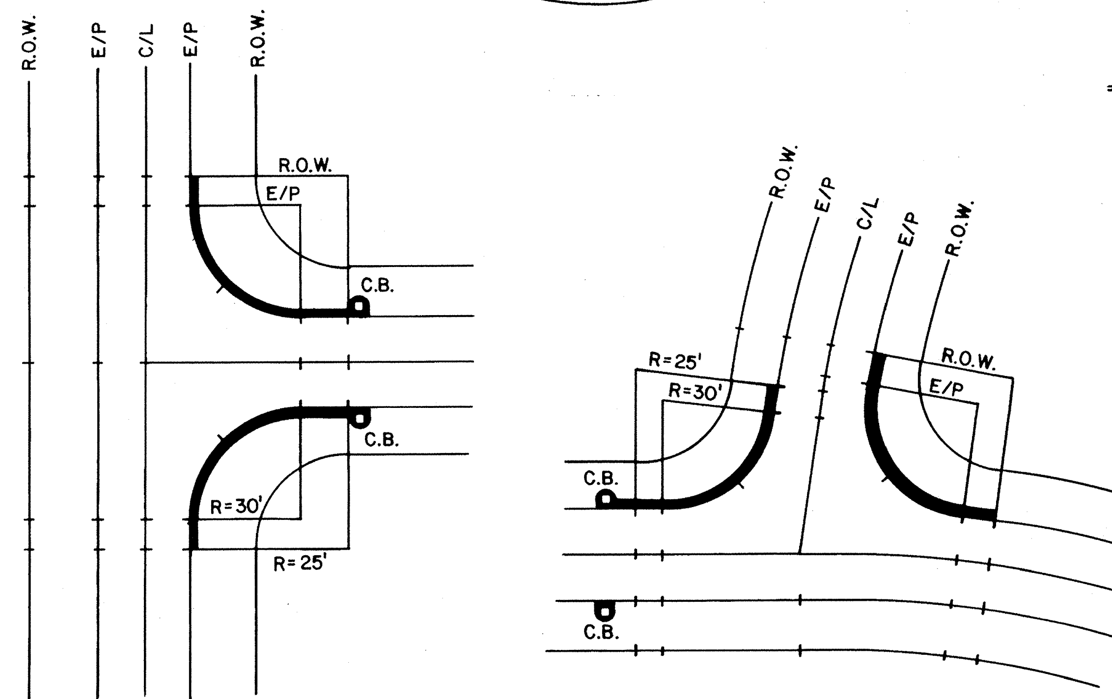
TYPICAL STREET AND CORNER CURVE LAYOUT
