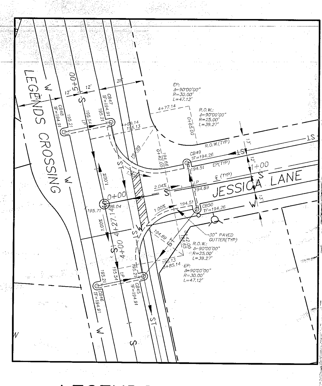
LEGENDS CROSSING & JESSICA LANE HOR: 1" = 30'
