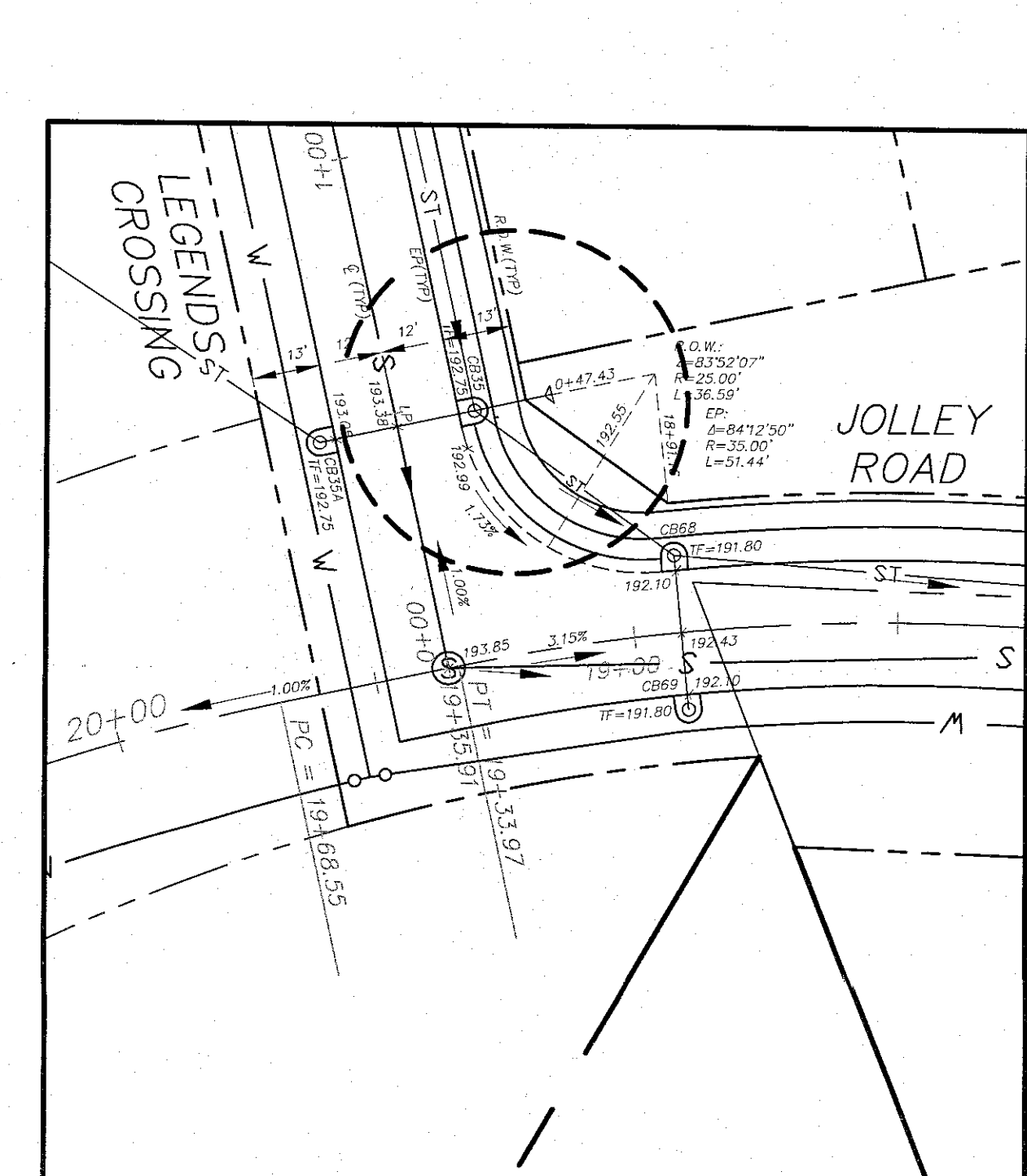
JOLLEY ROAD & LEGENDS CROSSING HOR: 1" = 30'
