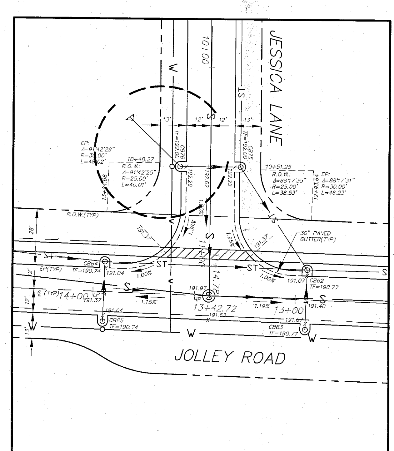
JOLLEY ROAD & JESSICA LANE HOR: 1" = 30'
