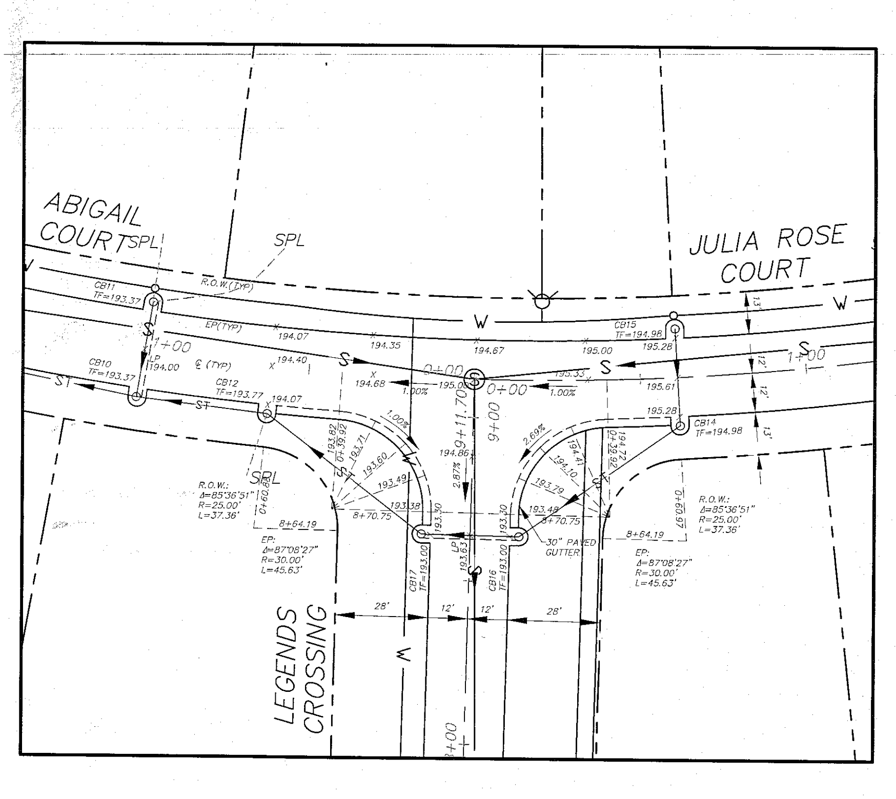
LEGENDS CROSSING & ABIGAIL/JULIA ROSE COURT'S HOR: 1" = 30'
