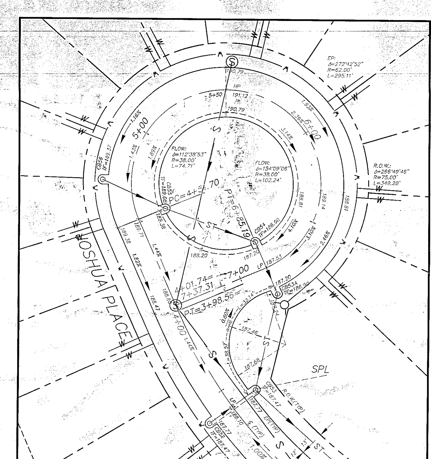
JOSHUA PLACE CUL-DE-SAC HOR: 1" = 30'
