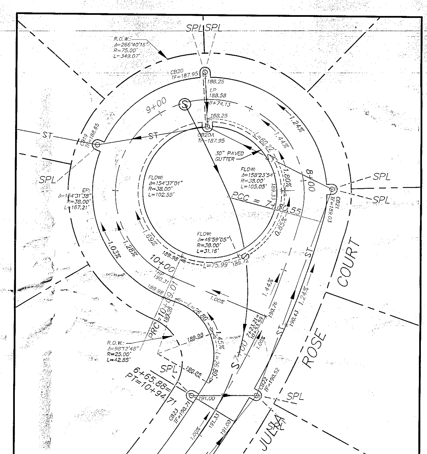
JULIA ROSE COURT CUL-DE-SAC HOR: 1" = 30'
