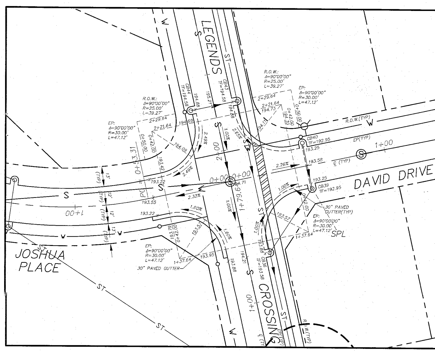
LEGENDS CROSSING & JOSHUA PLACE/DAVID DRIVE HOR: 1" = 30'
