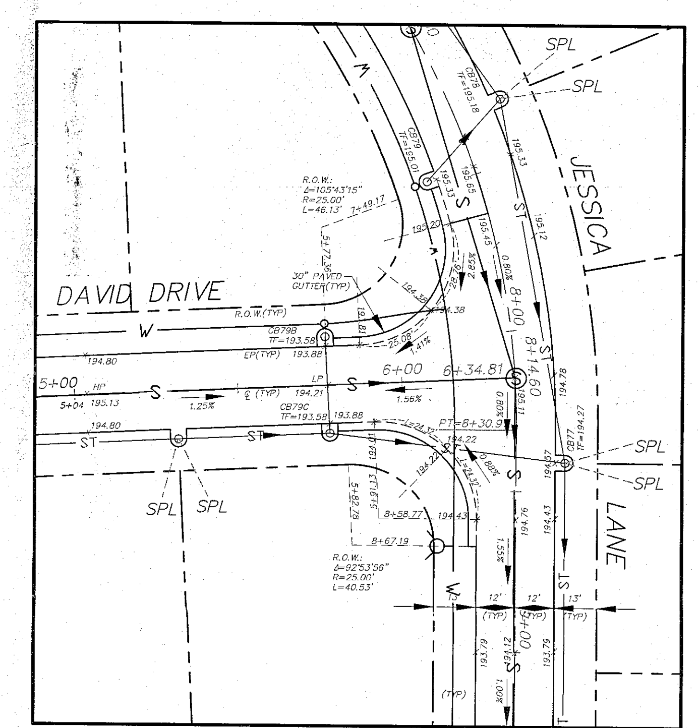
DAVID DRIVE & JESSICA LANE HOR: 1" = 30'
