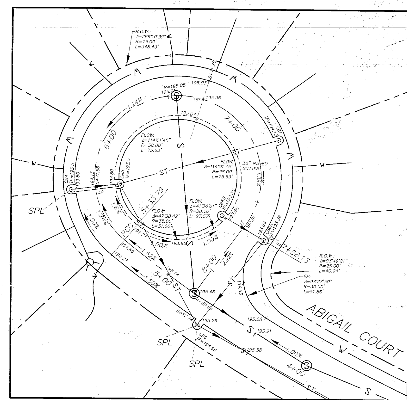
ABIGAIL COURT CUL-DE-SAC HOR: 1" = 30'
