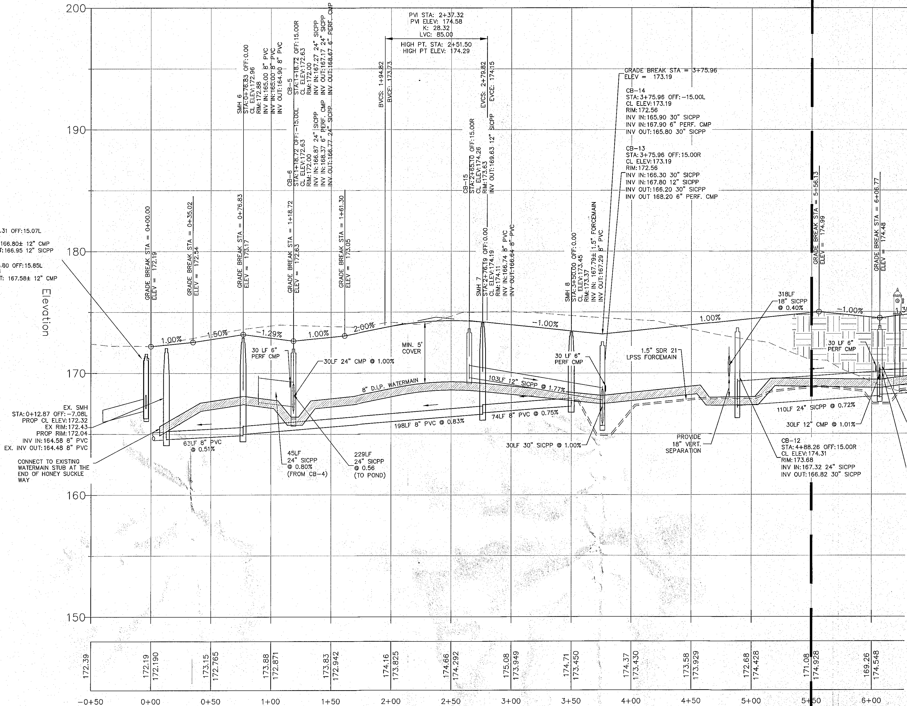
HONEY SUCKLE WAY PROFILE MATCH SHEET 11 SCALE: 1" = 40' HORIZONTAL 1" = 4' VERTICAL
