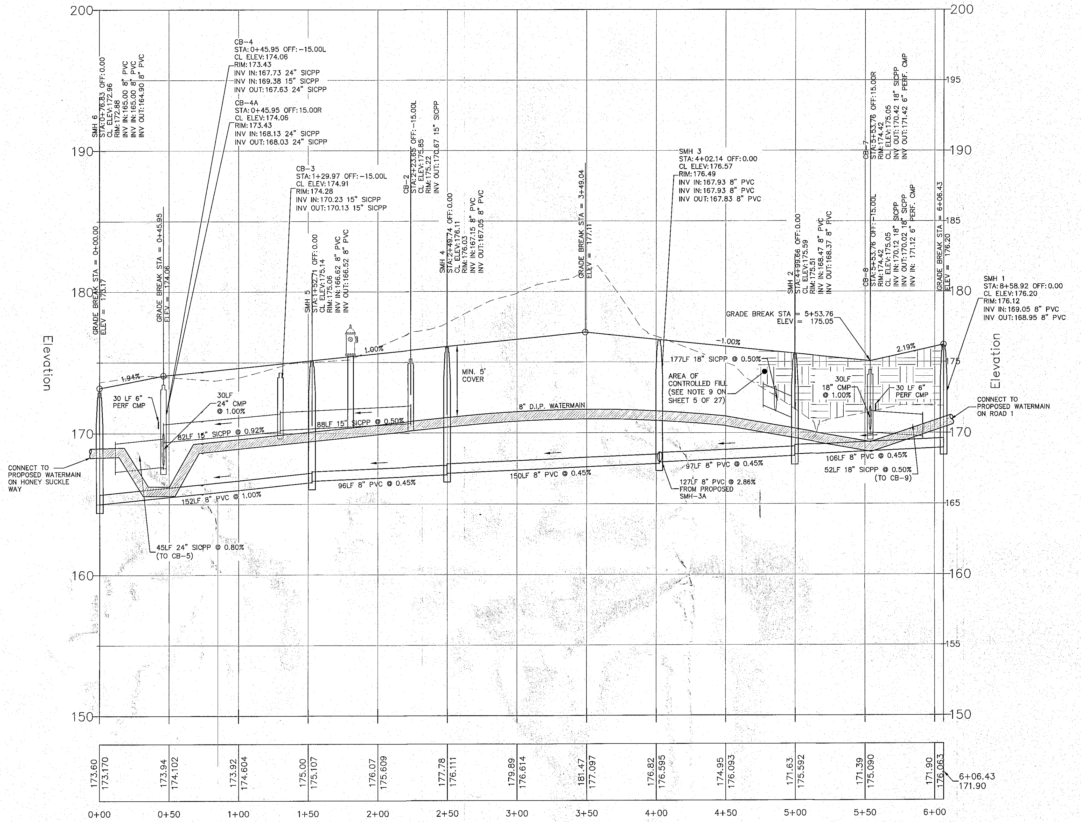
TWINFLOWER COURT PROFILE SCALE: 1"=40' HORIZONTAL 1"=4' VERTICAL
