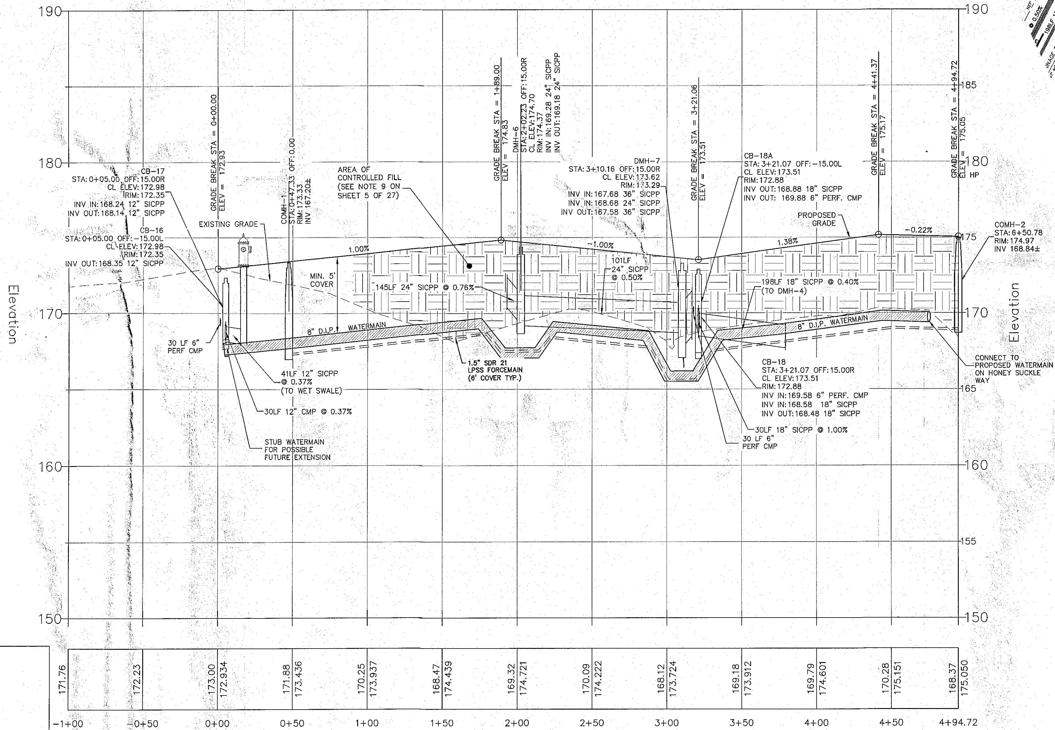
NEWELL LANE PROFILE SCALE: 1" = 40' HORIZONTAL 1" = 4' VERTICAL
