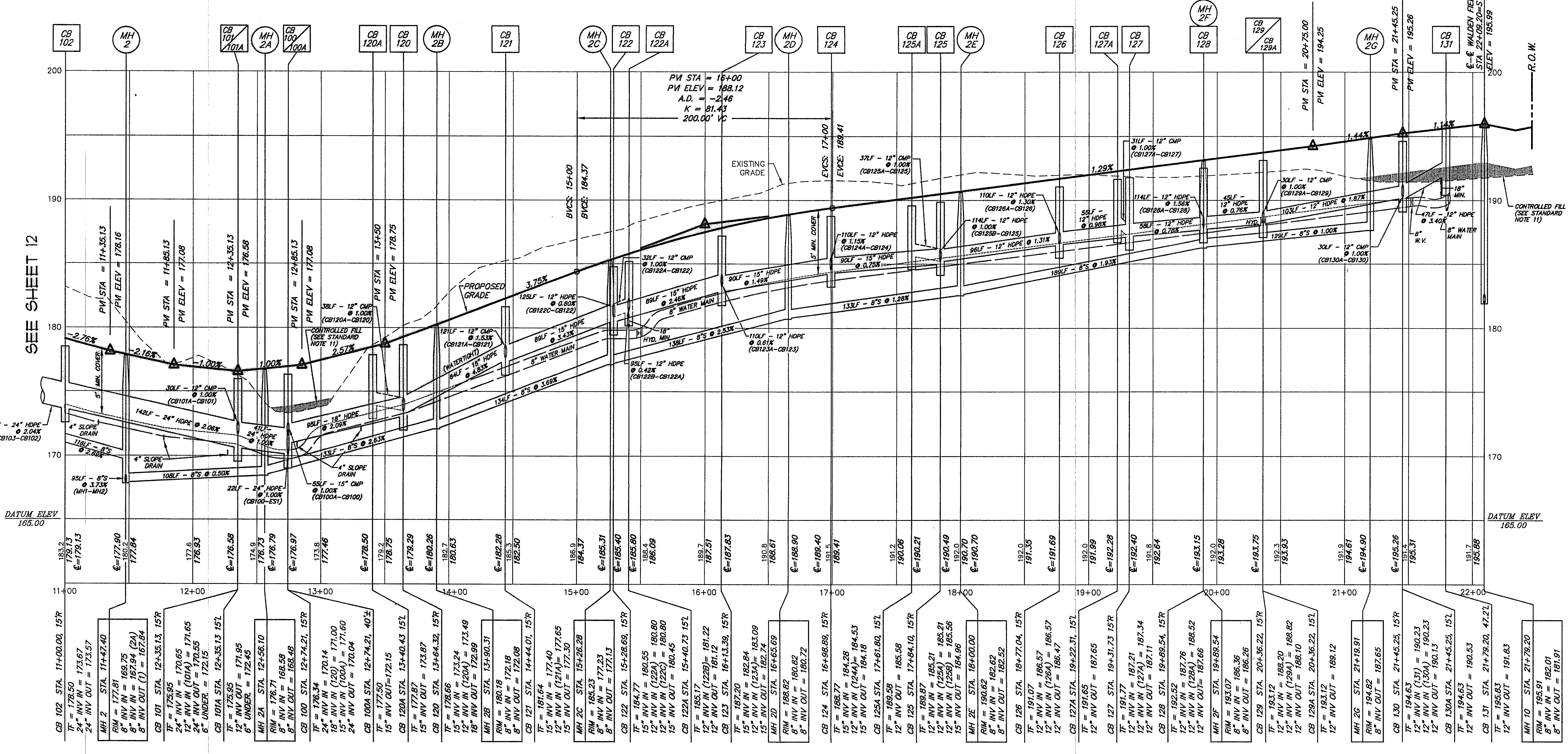
PROFILE SCALE: 1" = 50' HORZ. 1" = 5' VERT. (WALDEN FIELDS DRIVE) (STA 11+00 TO 22+09.20)
