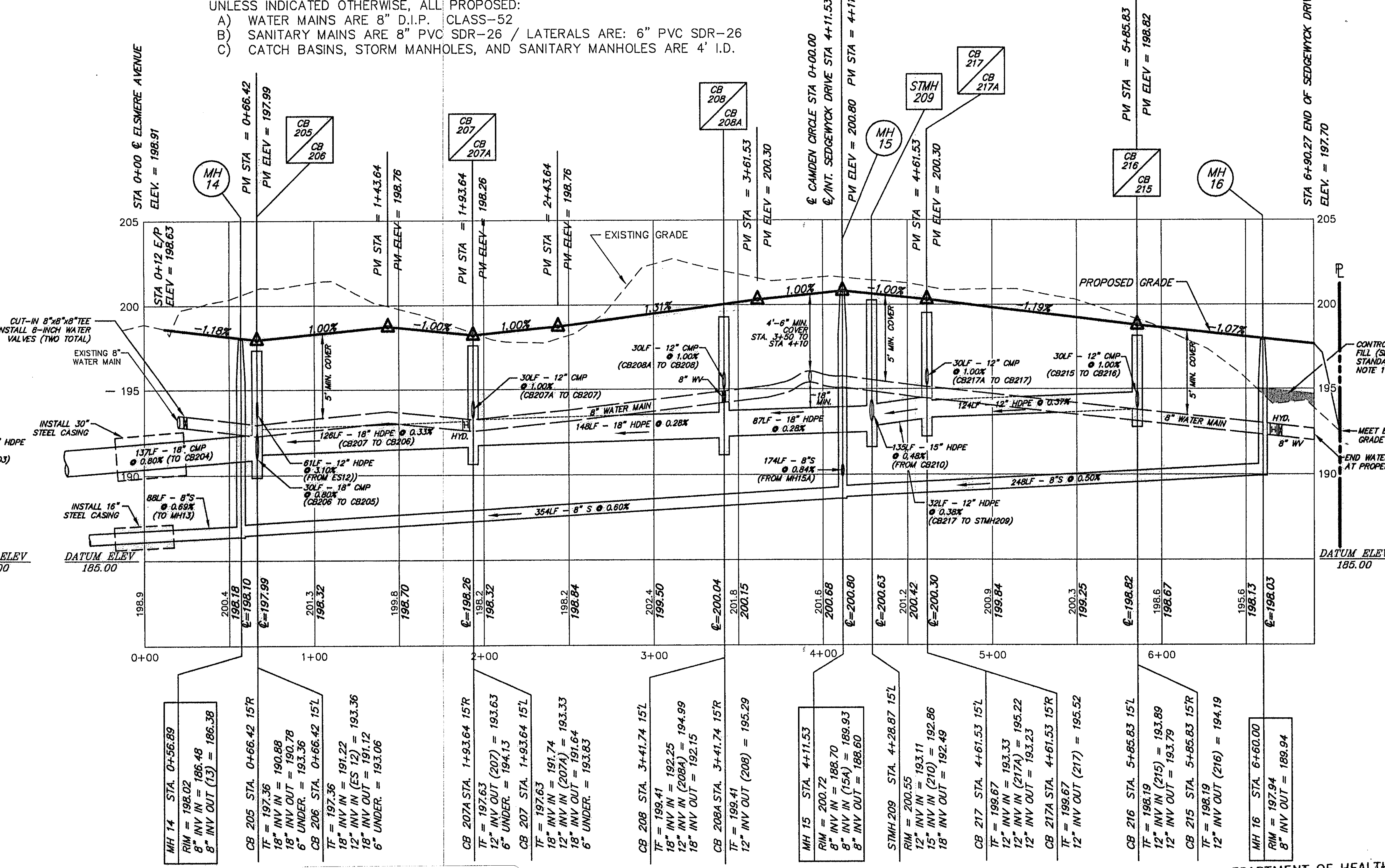
PROFILE SCALE: 1" = 50' HORIZ. (SEDGEWYCK DRIVE - STA 0+00 TO 6+90.27)
