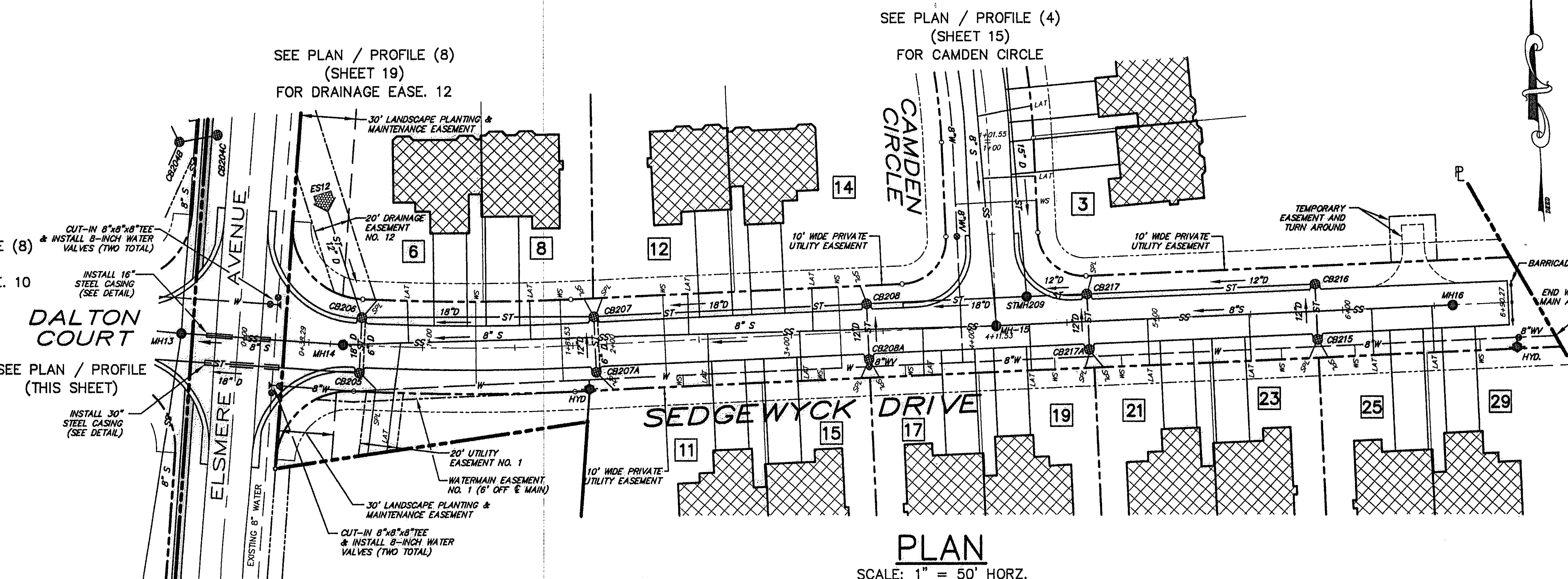
PLAN SCALE: 1" = 50' HORIZ. (SEDGEWYCK DRIVE - STA 0+00 TO 6+90.27)
