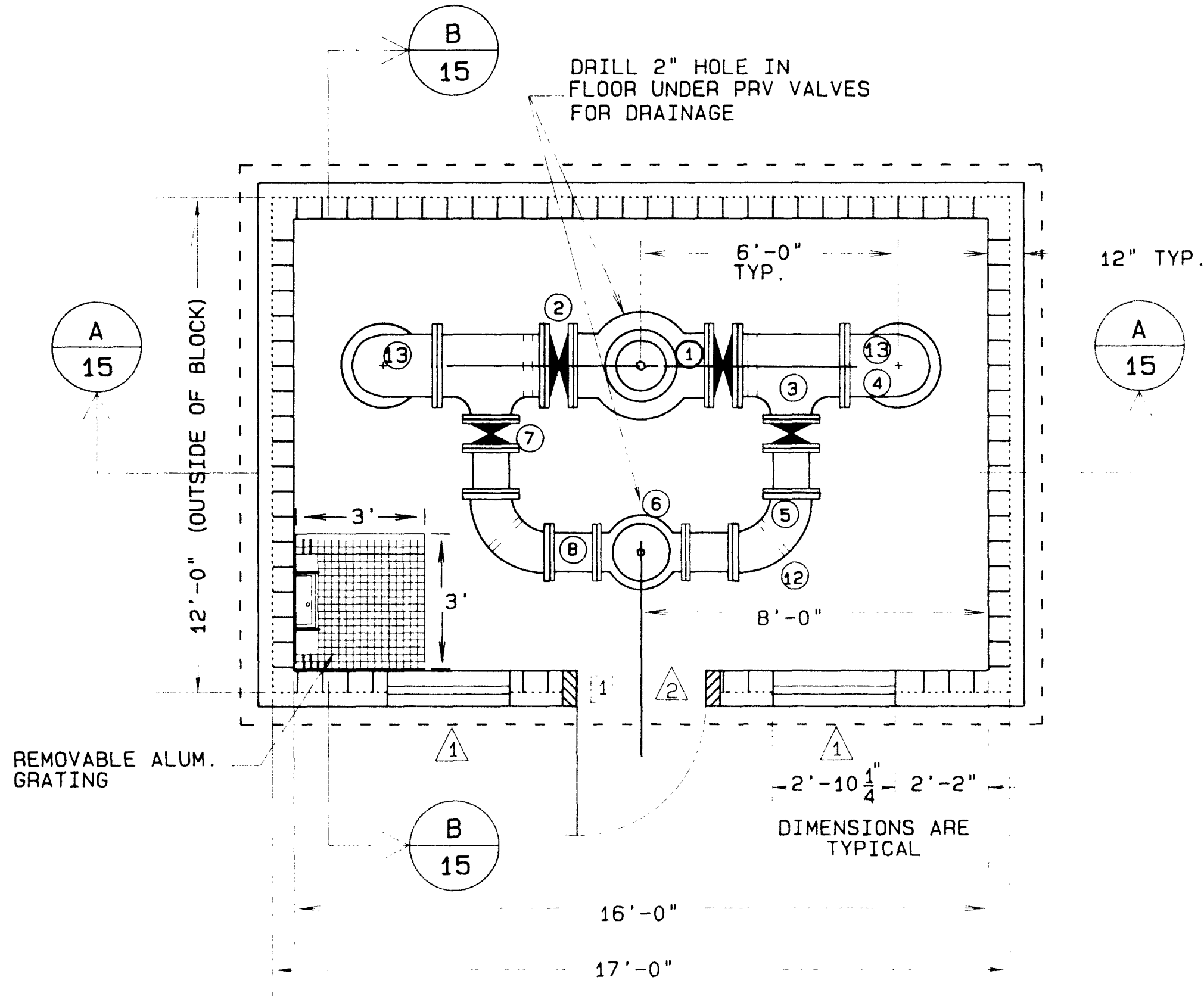
PRV STATION PLAN SCALE: 3/8"=1'-0"
