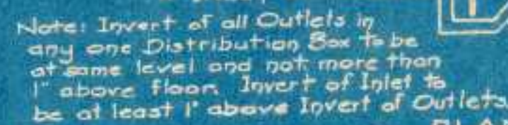
PLAN DISTRIBUTION BOX Scale \frac{1}{4}" = 1'
