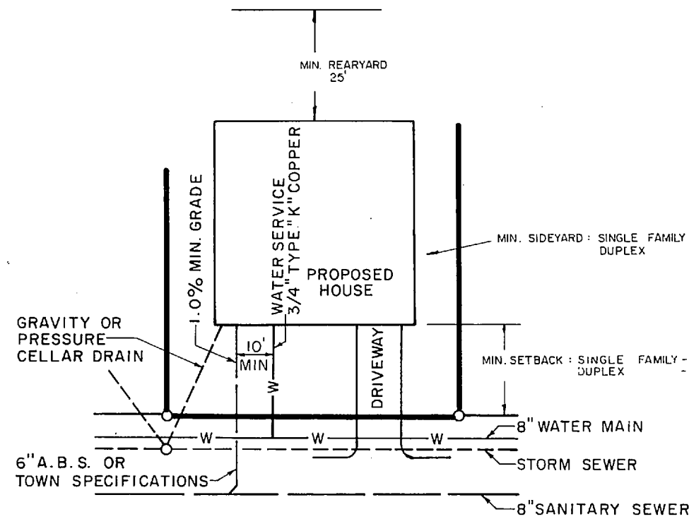
TYPICAL LOT LAYOUT (NOT TO SCALE)
