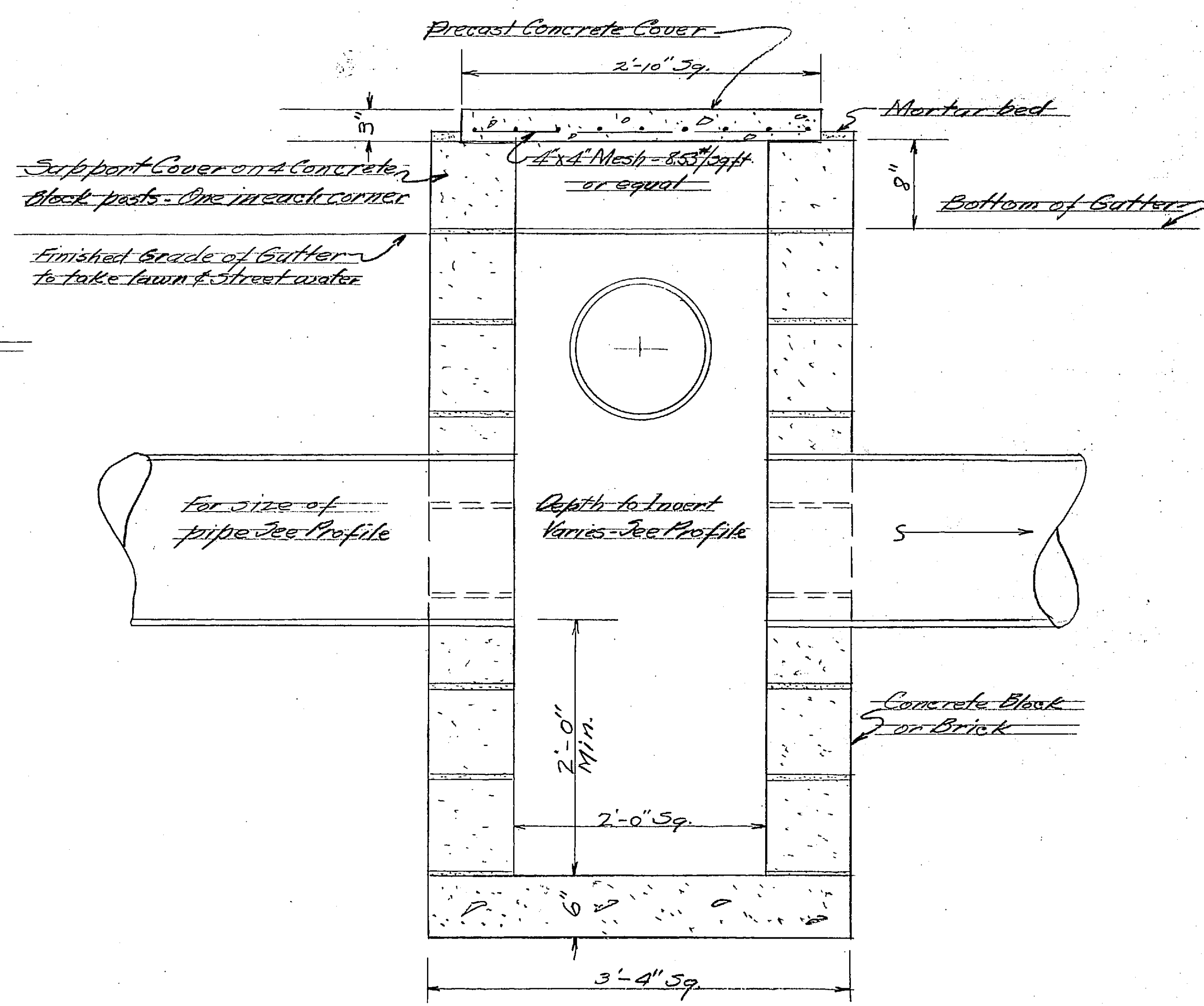
- TYPICAL SECTION - - CATCH BASIN - SCALE 1" = 1'-0"
