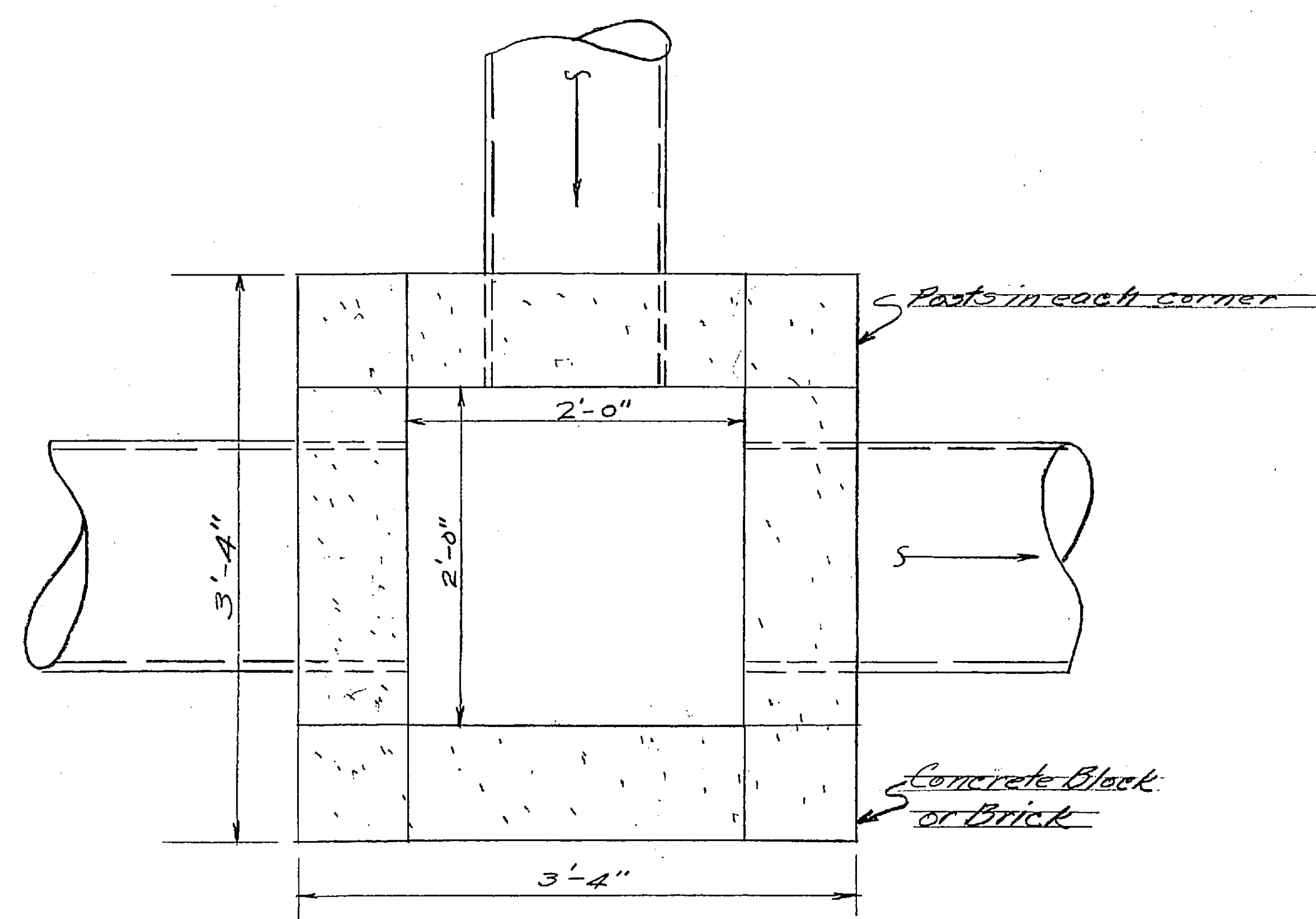
- PLAN OF CATCH BASIN - SCALE 1" = 1'-0"
