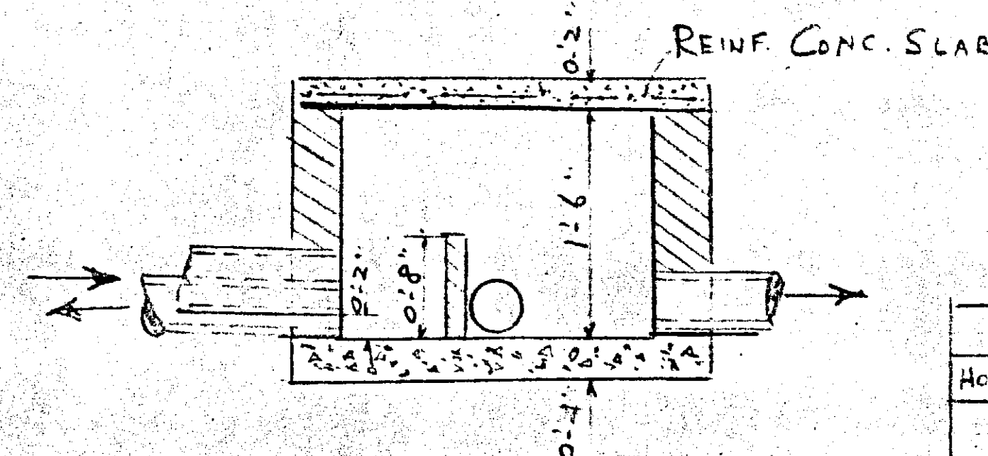
HORIZONTAL SECTION VERTICAL SECTION DETAIL OF DISTRIBUTION BOX SCALE 3/4\"/>
