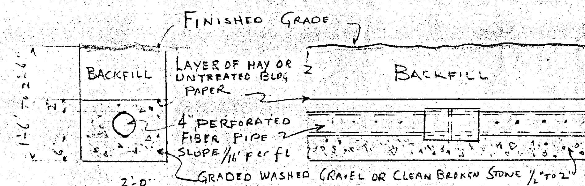
CROSS SECTION LONGITUDINAL SECTION DETAIL OF TILE FIELD TRENCH NOT TO SCALE
