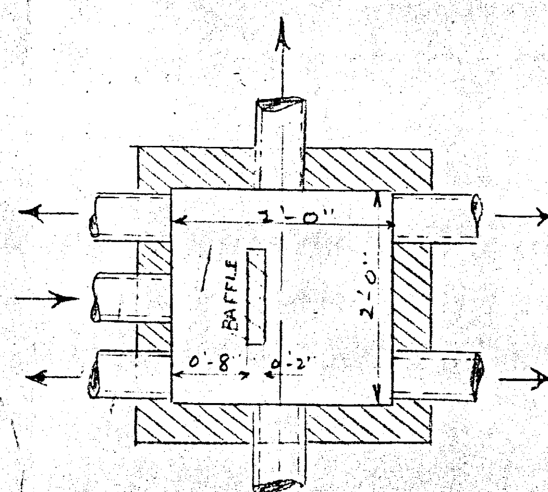
HORIZONTAL SECTION VERTICAL SECTION DETAIL OF DISTRIBUTION BOX SCALE 3/4\"/>
