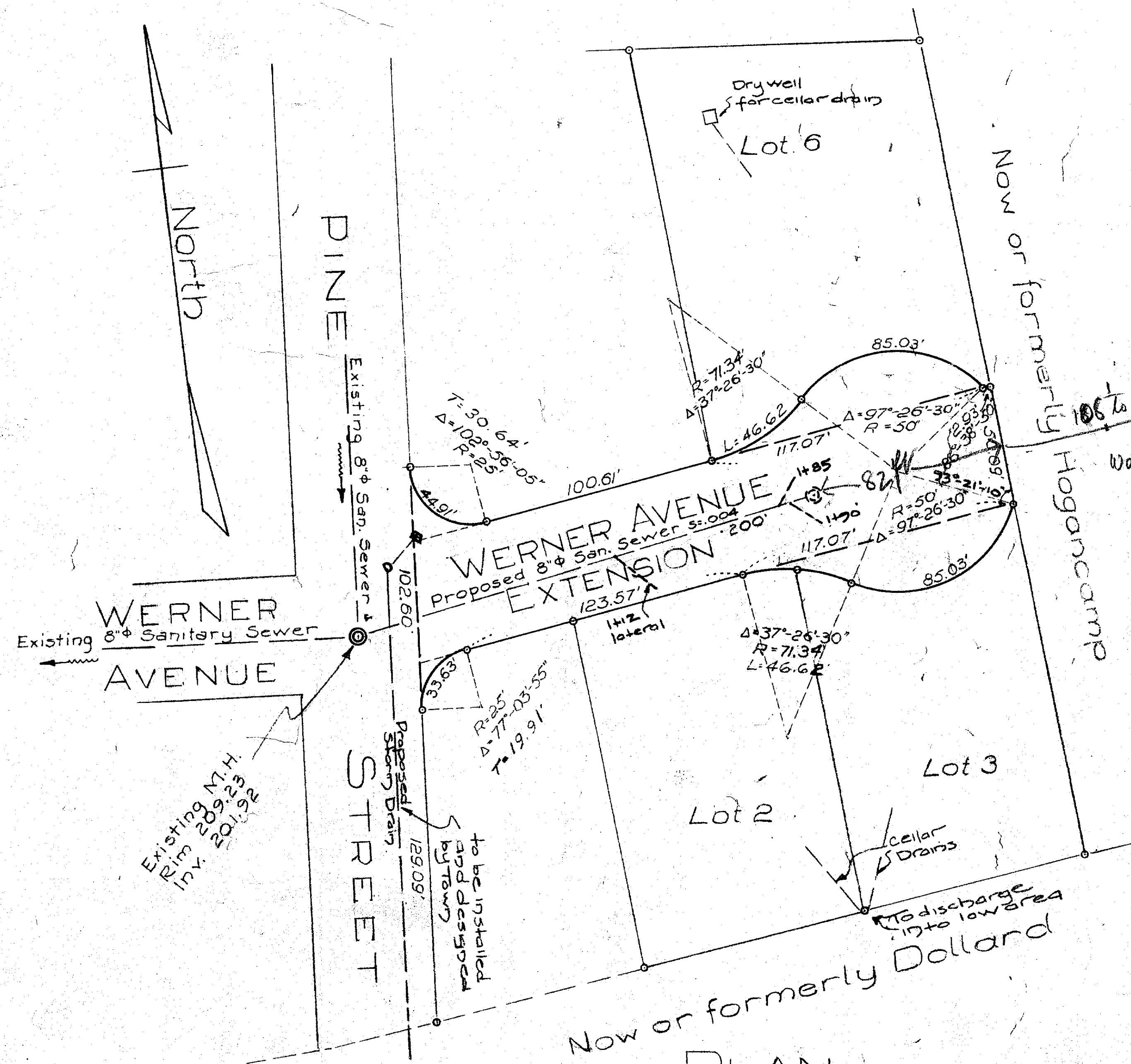
PLAN Scale 1" = 50'
