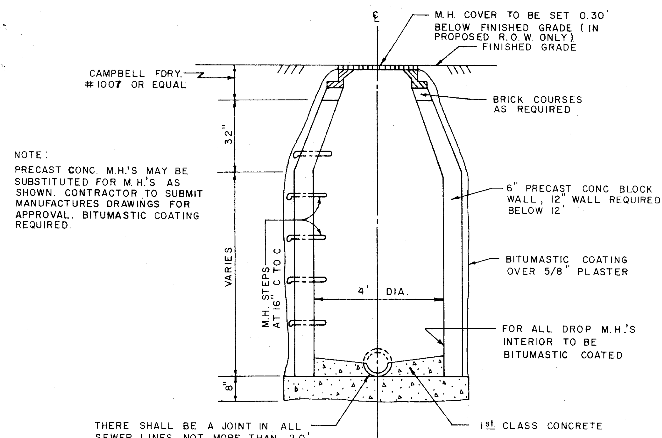
STANDARD MANHOLE NOT TO SCALE
