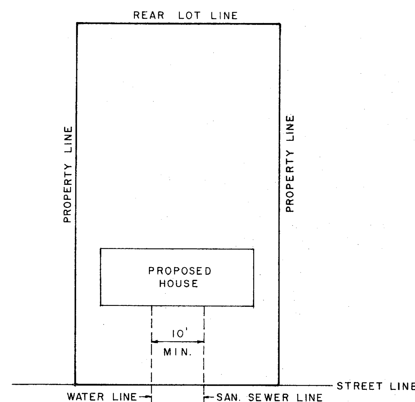
TYPICAL LOT LAYOUT SCALE: 1" = 40'
