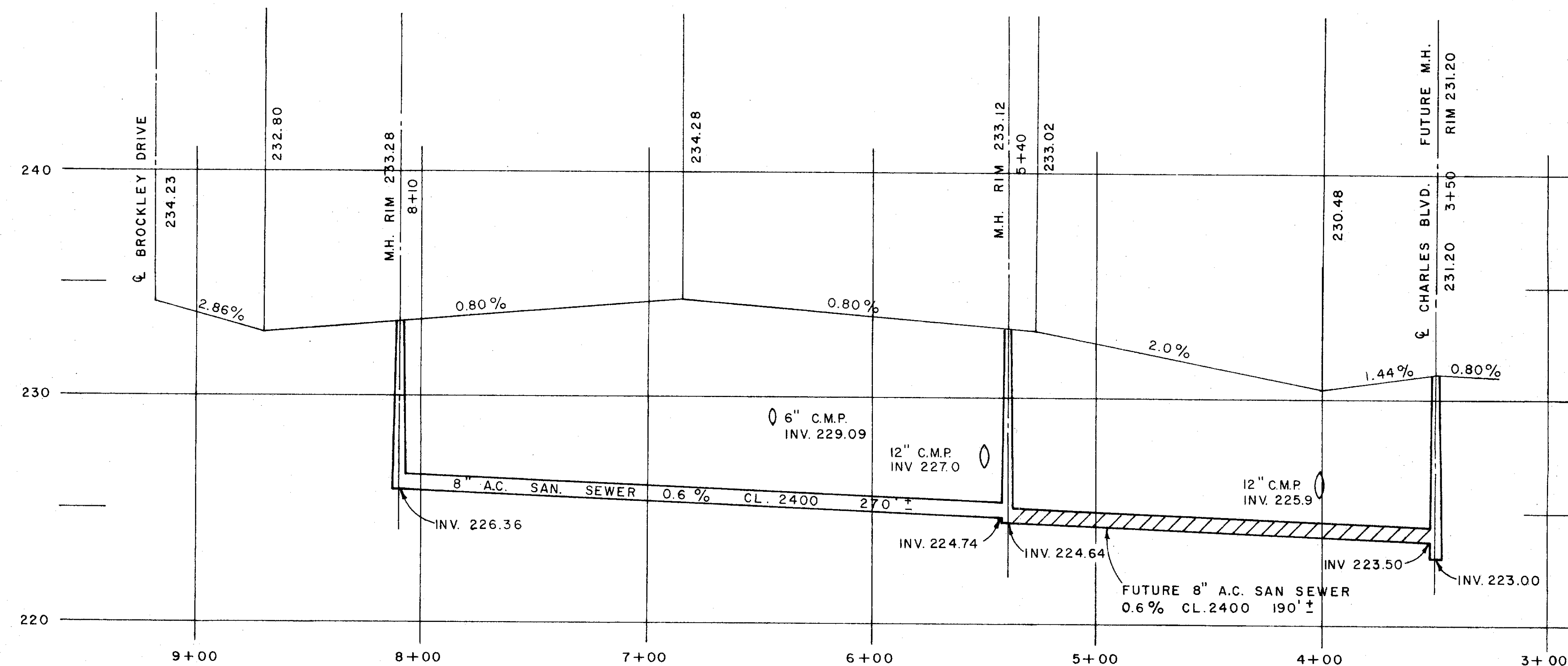
PROFILE SCALE: HORZ. 1" = 50' VERT. 1" = 5'
