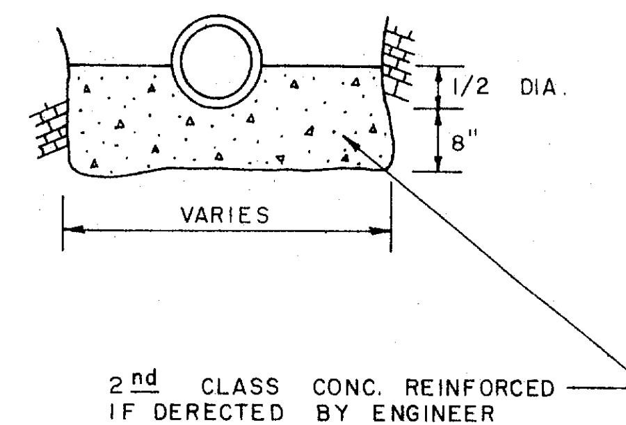
CONCRETE PIPE CRADLE NOT TO SCALE
