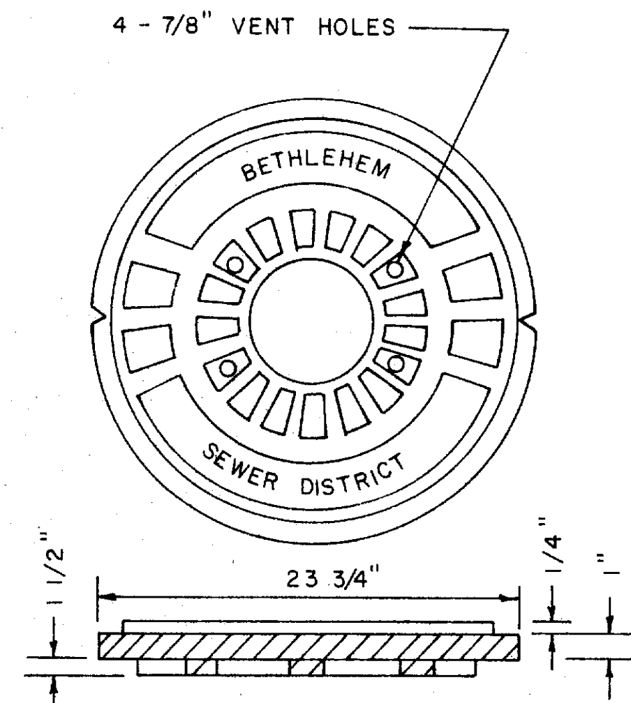
STANDARD MANHOLE COVER NOT TO SCALE
