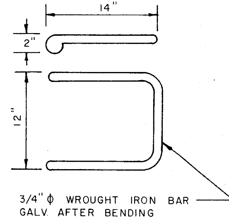
MANHOLE STEPS NOT TO SCALE
