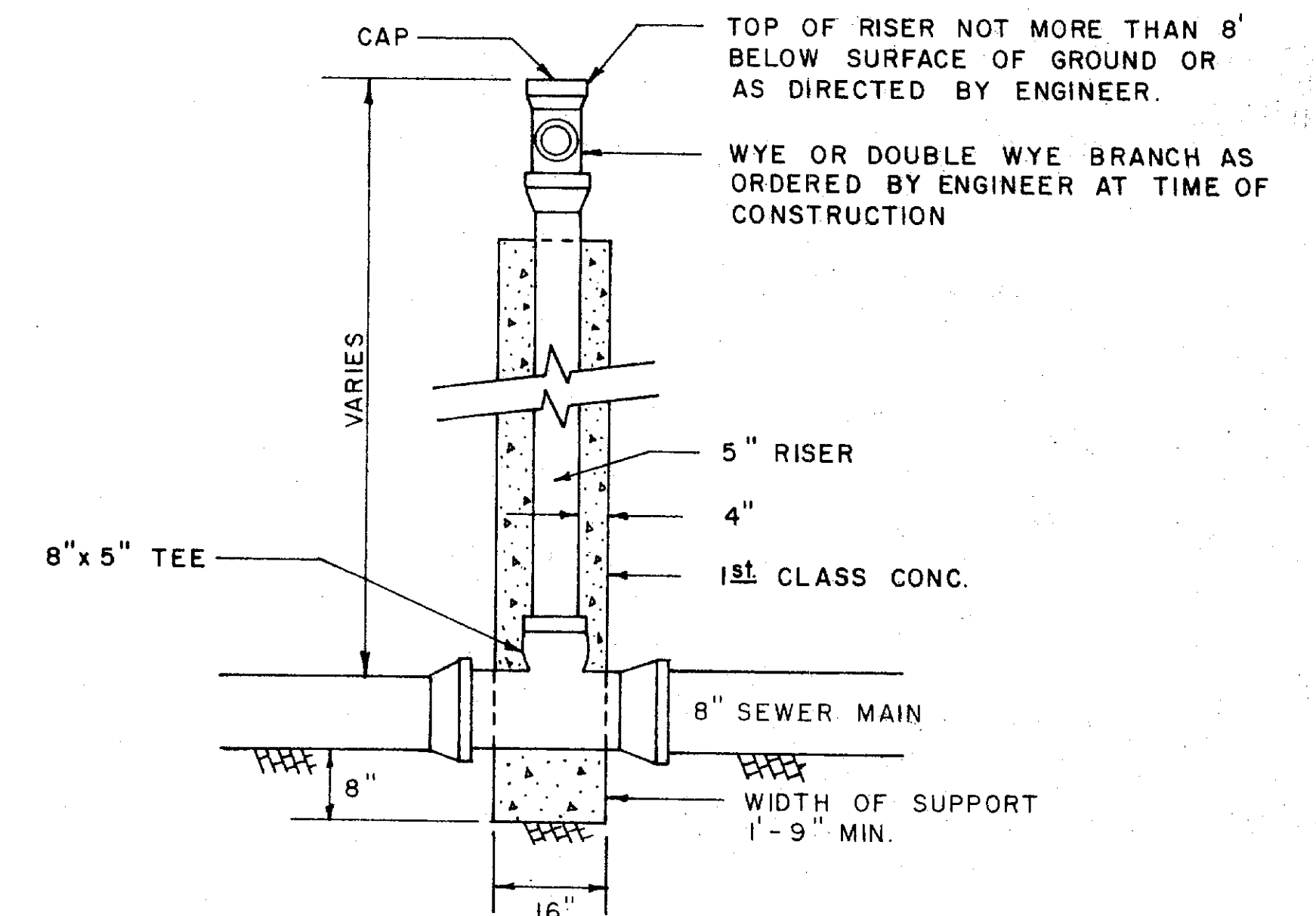
DETAIL OF VERTICAL PIPE RISER NOT TO SCALE
