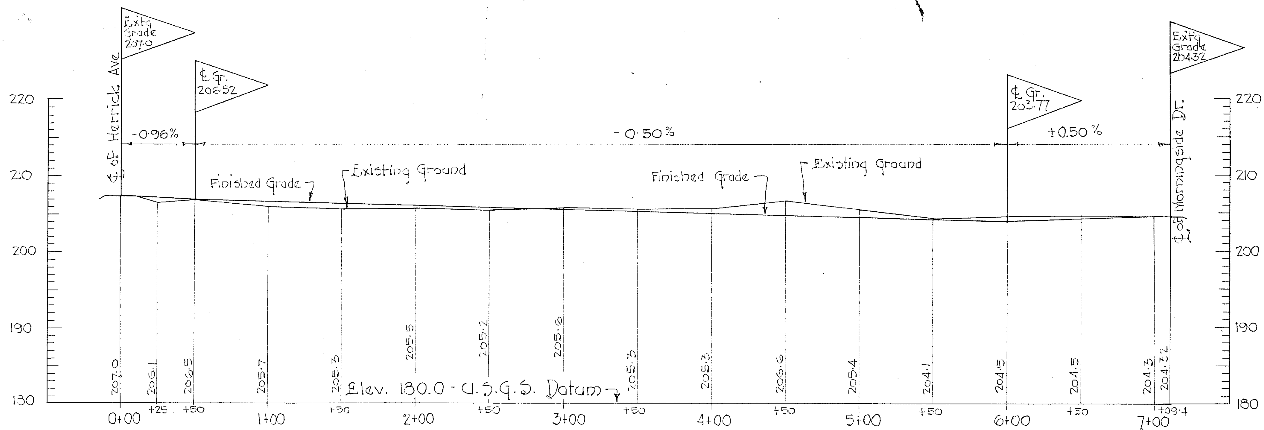
Profile of Park Place - along Center Line
