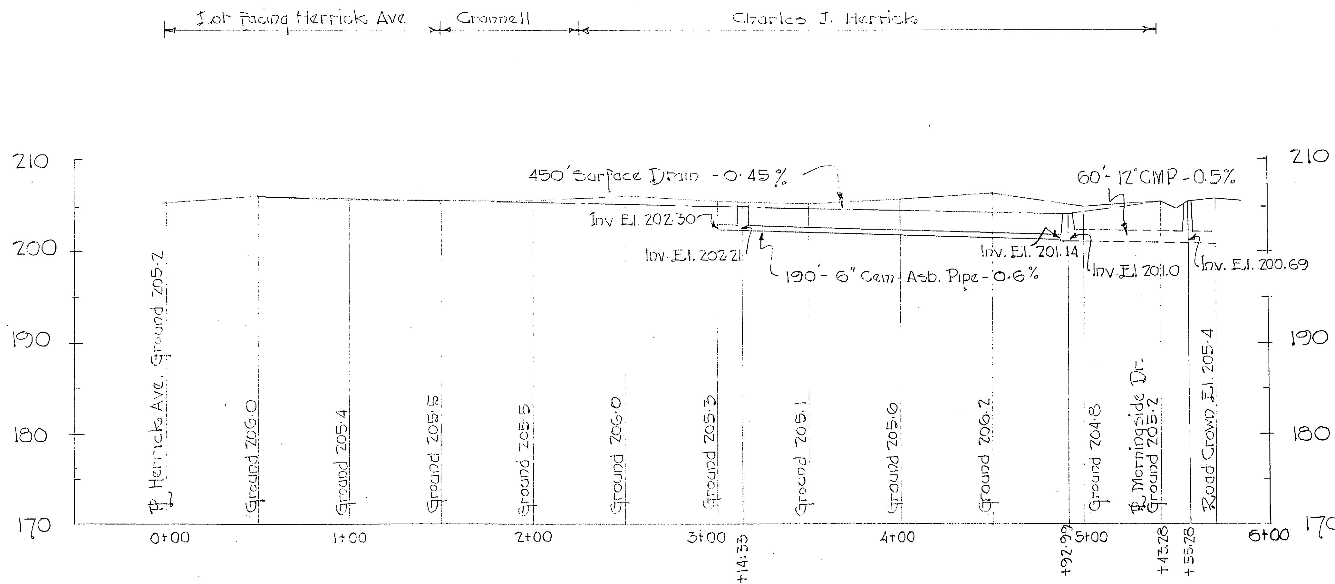
Profile of Surface & Foundation Drains along Southerly Lot Lines
