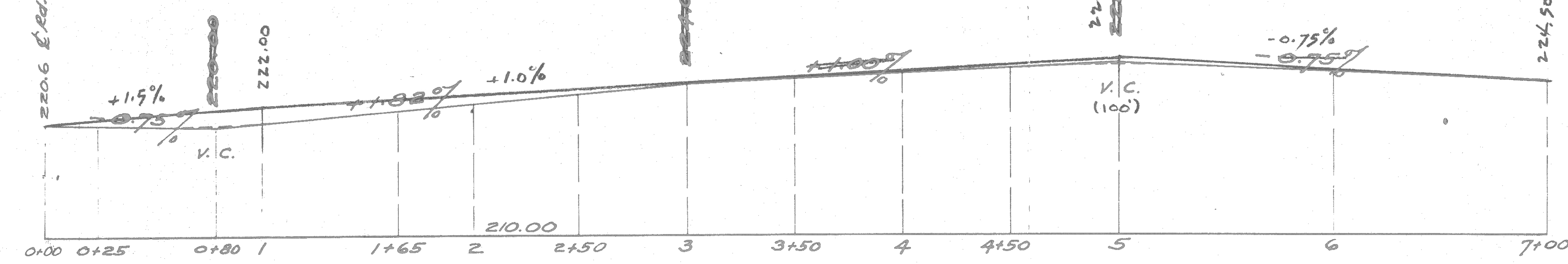
PROFILE ON CENTER LINE Scale: HOR. 1"=50' VER. 1"=10'
