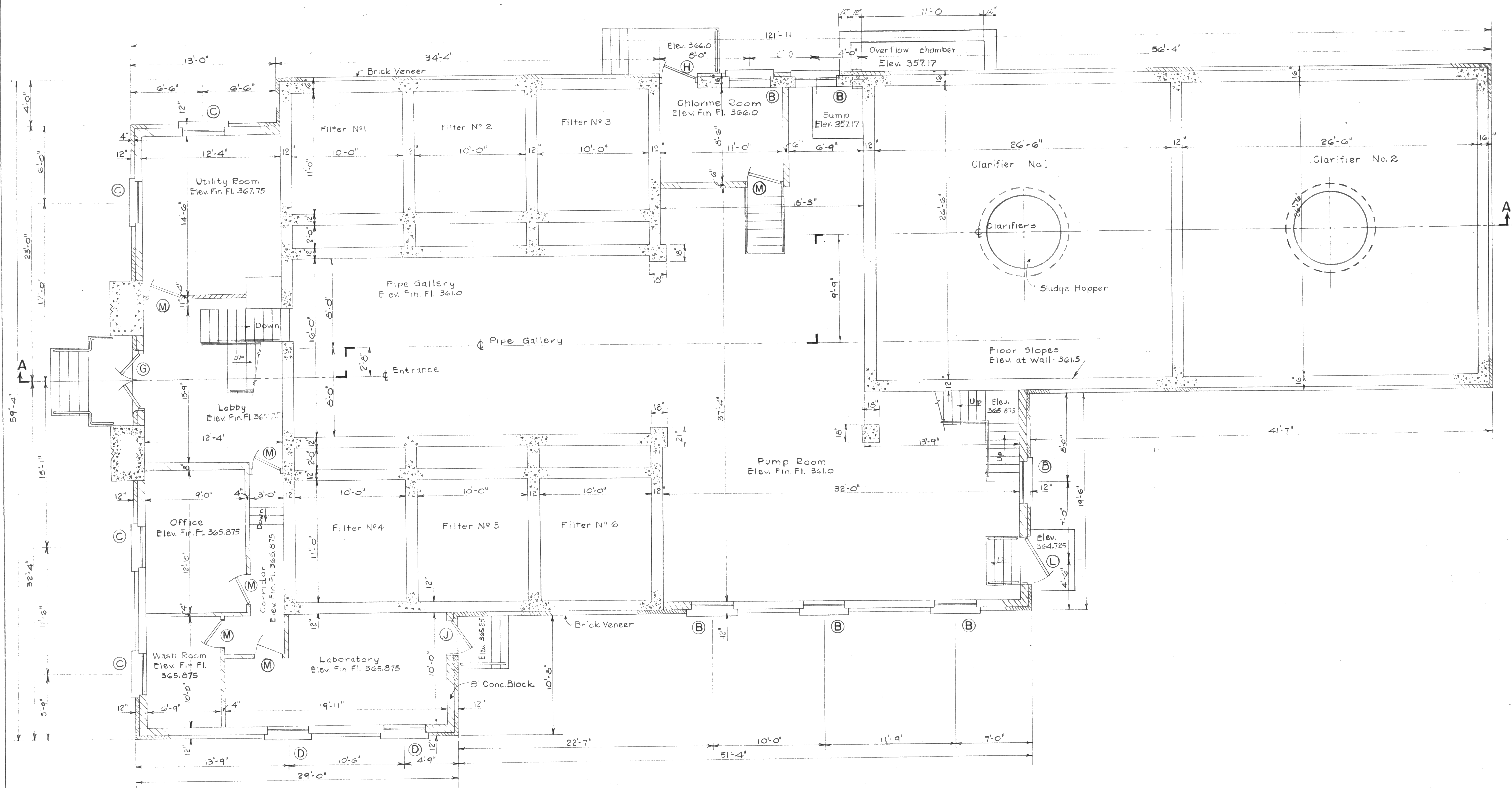
HORIZONTAL SECTION THROUGH BUILDING AT ELEV. 369.0 SCALE: \frac{1}{4}" = 1'-0"
